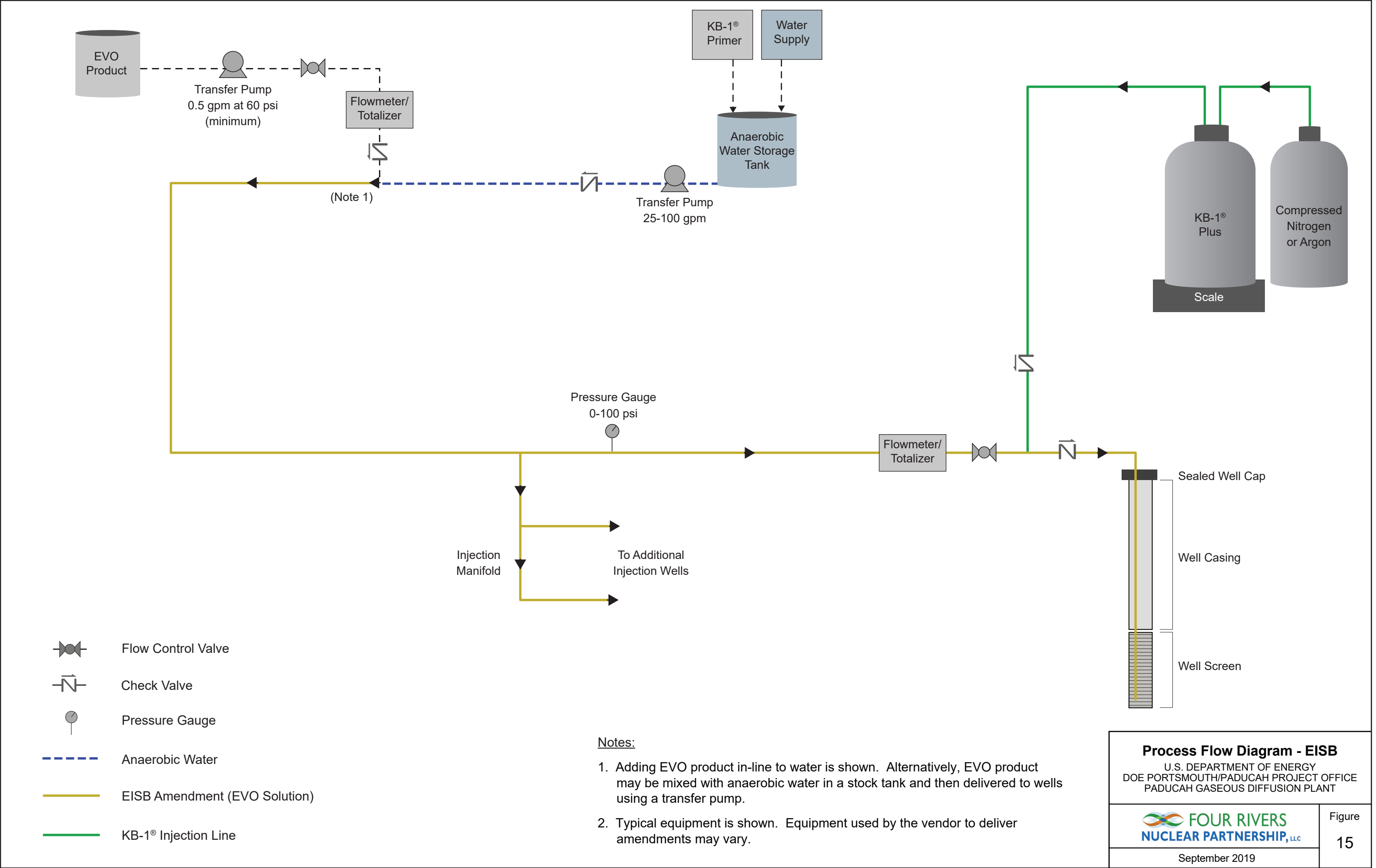
Figure 15. Process Flow Diagram - EISB
