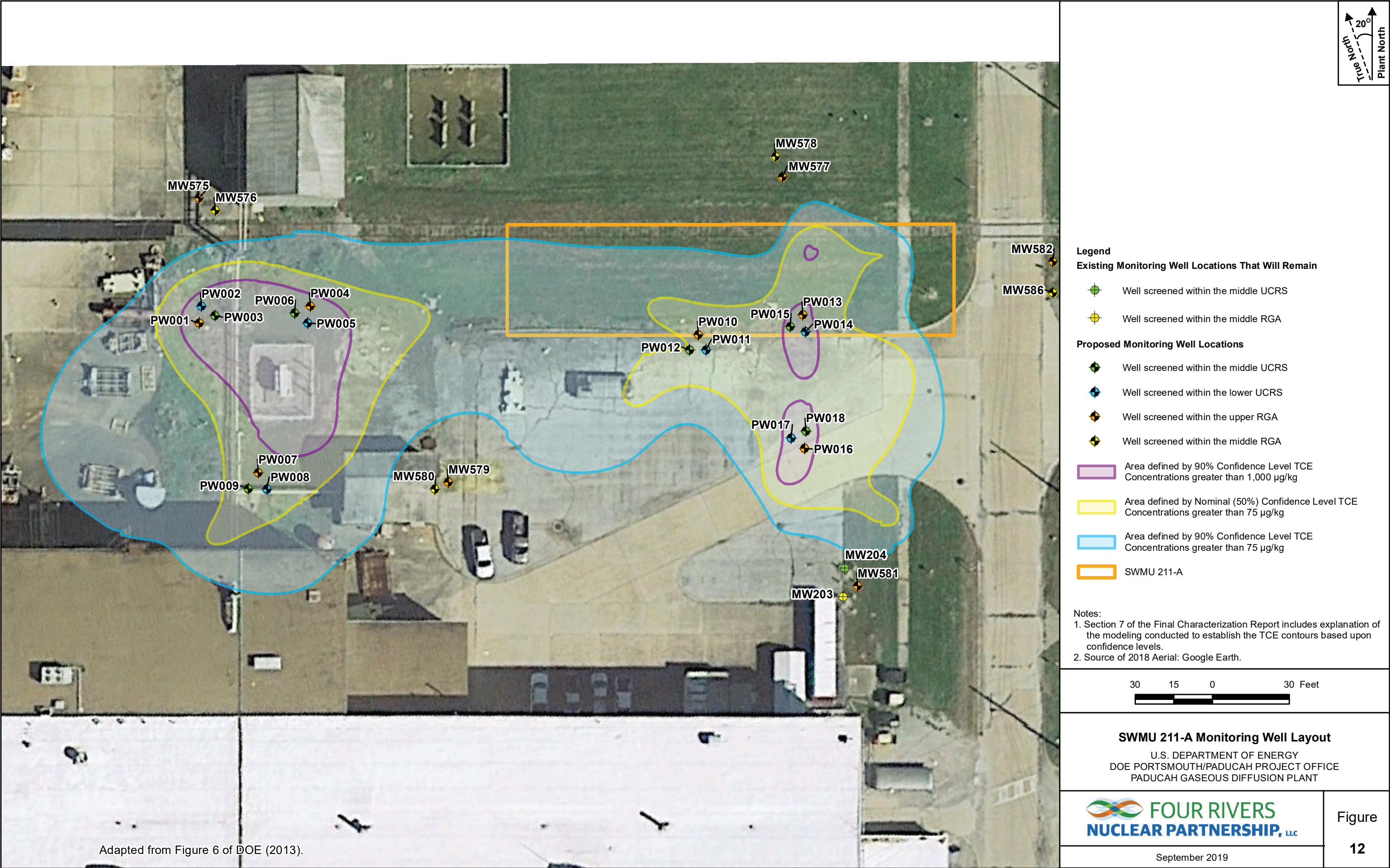
Figure 12. SWMU 211-A Monitoring Well Layout
