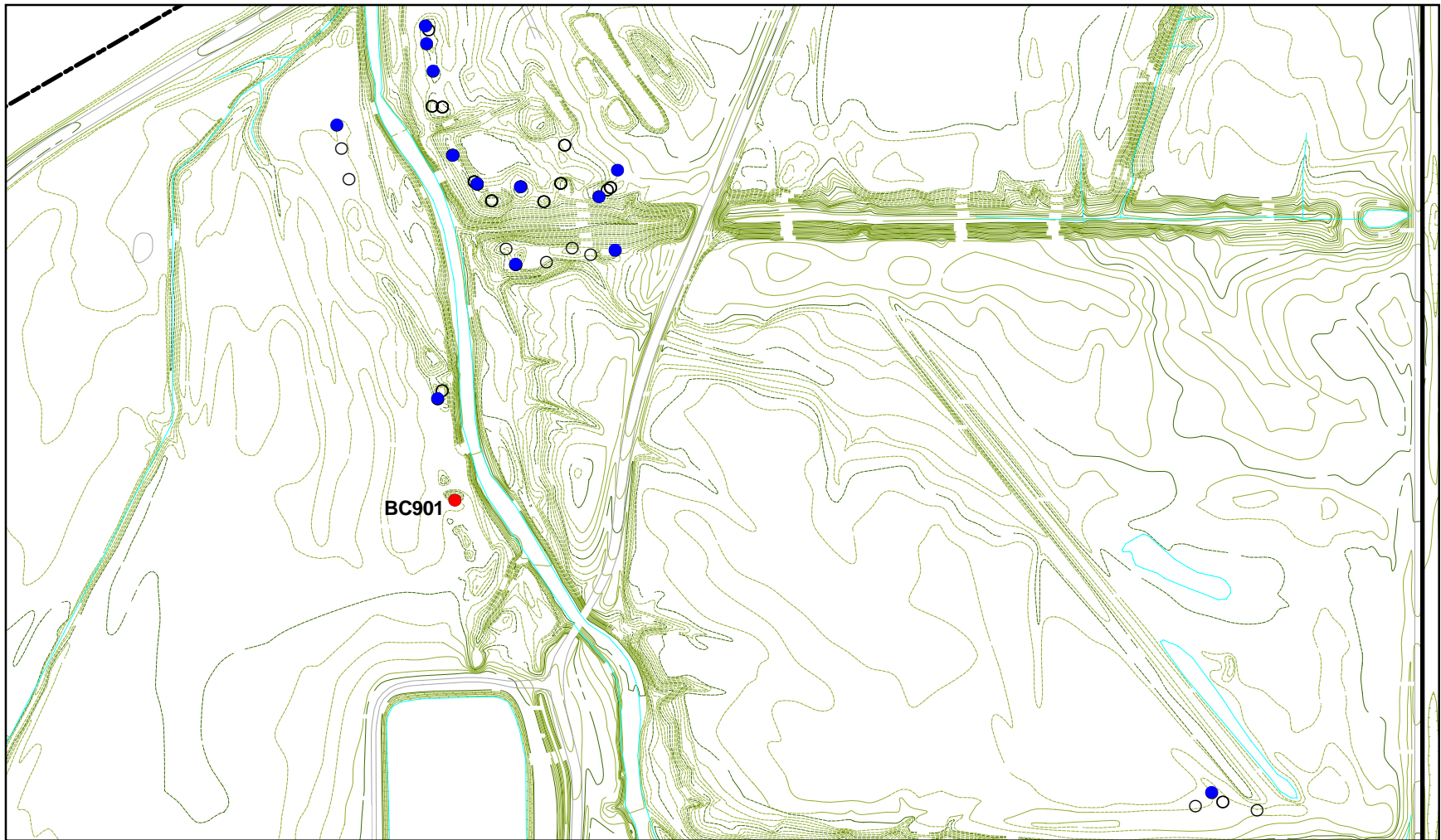
Figure B.16. (Continued) B-38
