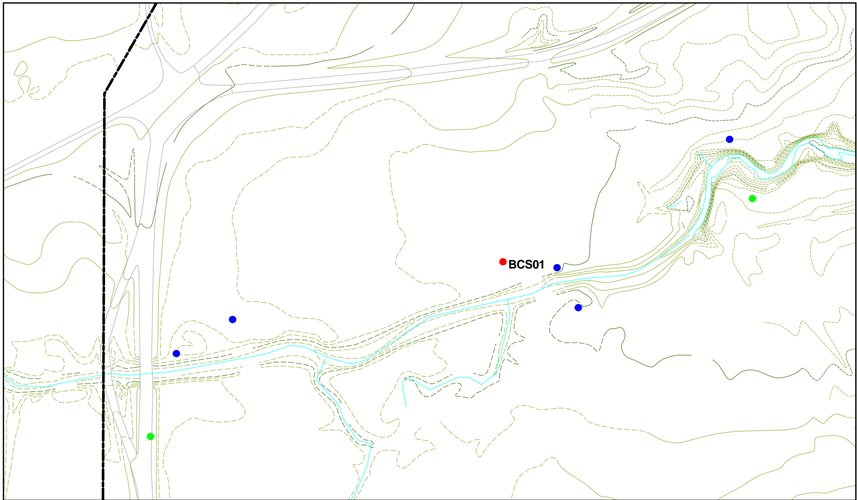
Figure B.6. (Continued) B-15
