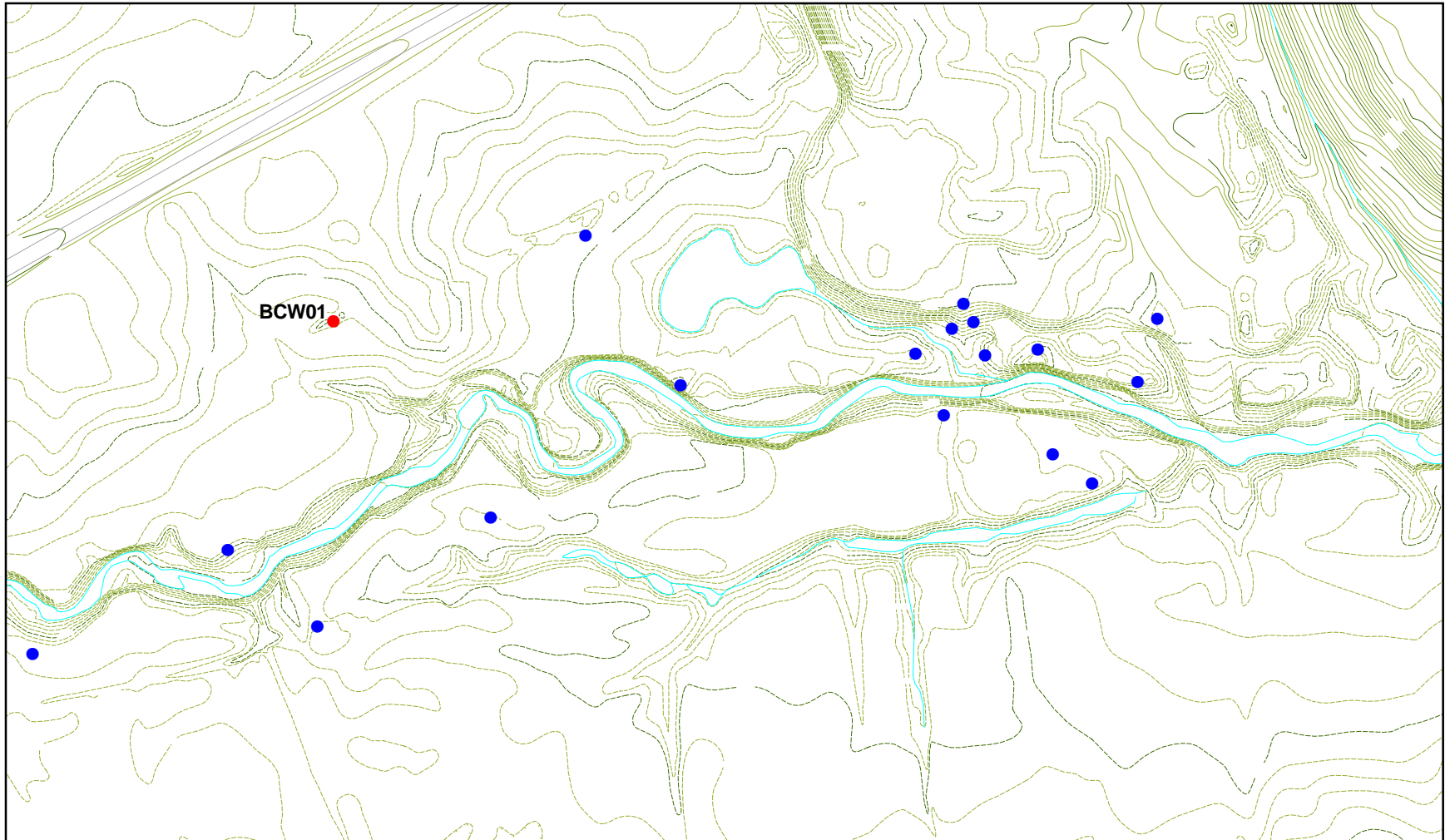
Figure B-20. (Continued) B-44
