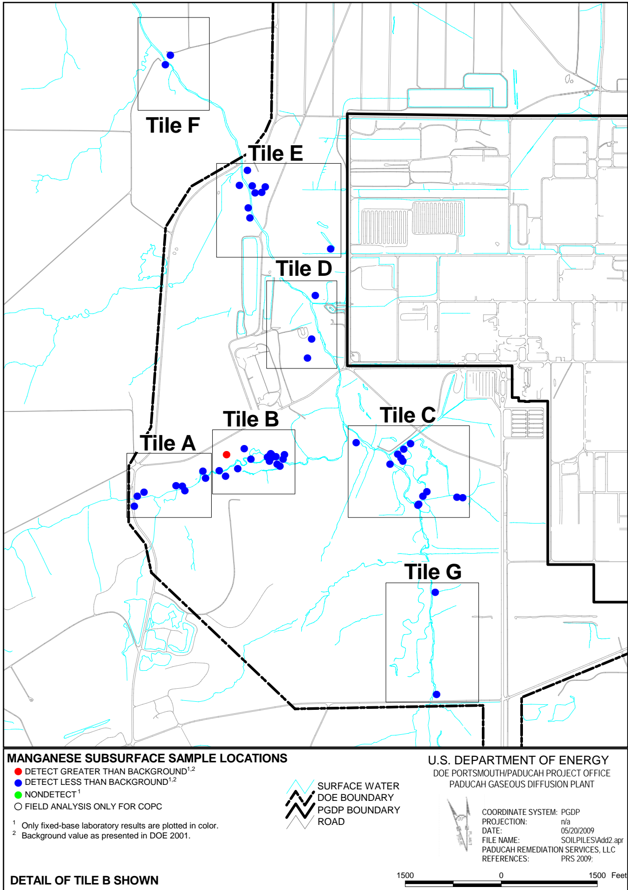
Figure B.20. Location of Sample Stations in Addendum 2 Soil Pile Sampling for Manganese in the Surface B-43
