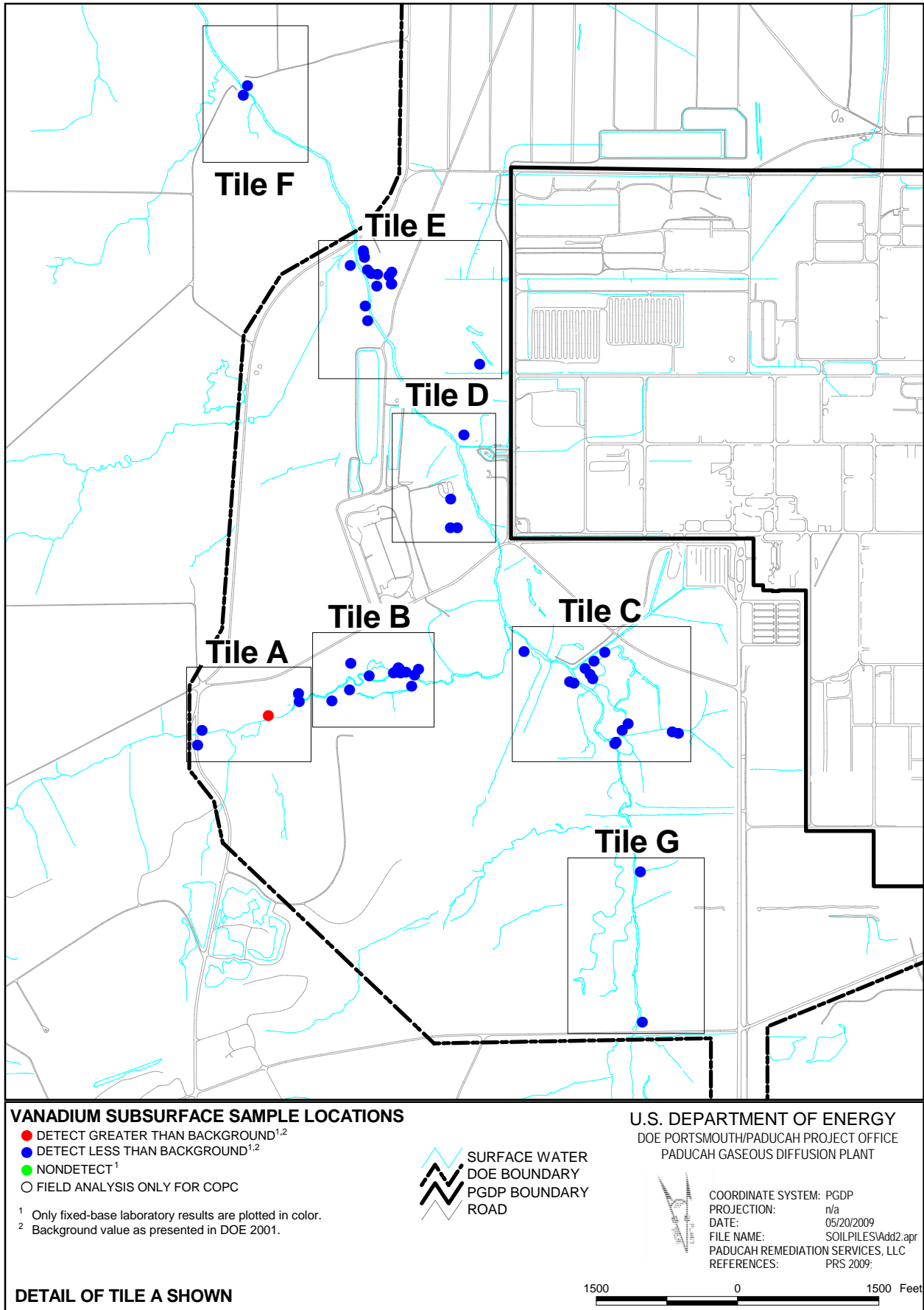
Figure B.22. Location of Sample Stations in Addendum 2 Soil Pile Sampling for Vanadium in the Subsurface B-46
