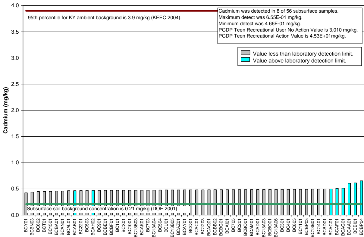
Figure B.9. Comparison between Cadmium Concentrations in Samples from Soil Piles Addendum 2 and Subsurface Soil Background Concentrations
