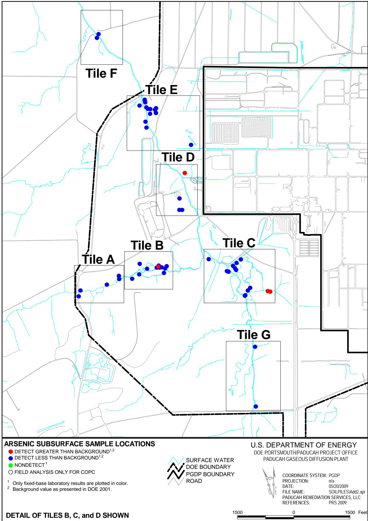
Figure B.4. Location of Sample Stations in Addendum 2 Soil Pile Sampling for Arsenic in the Subsurface
