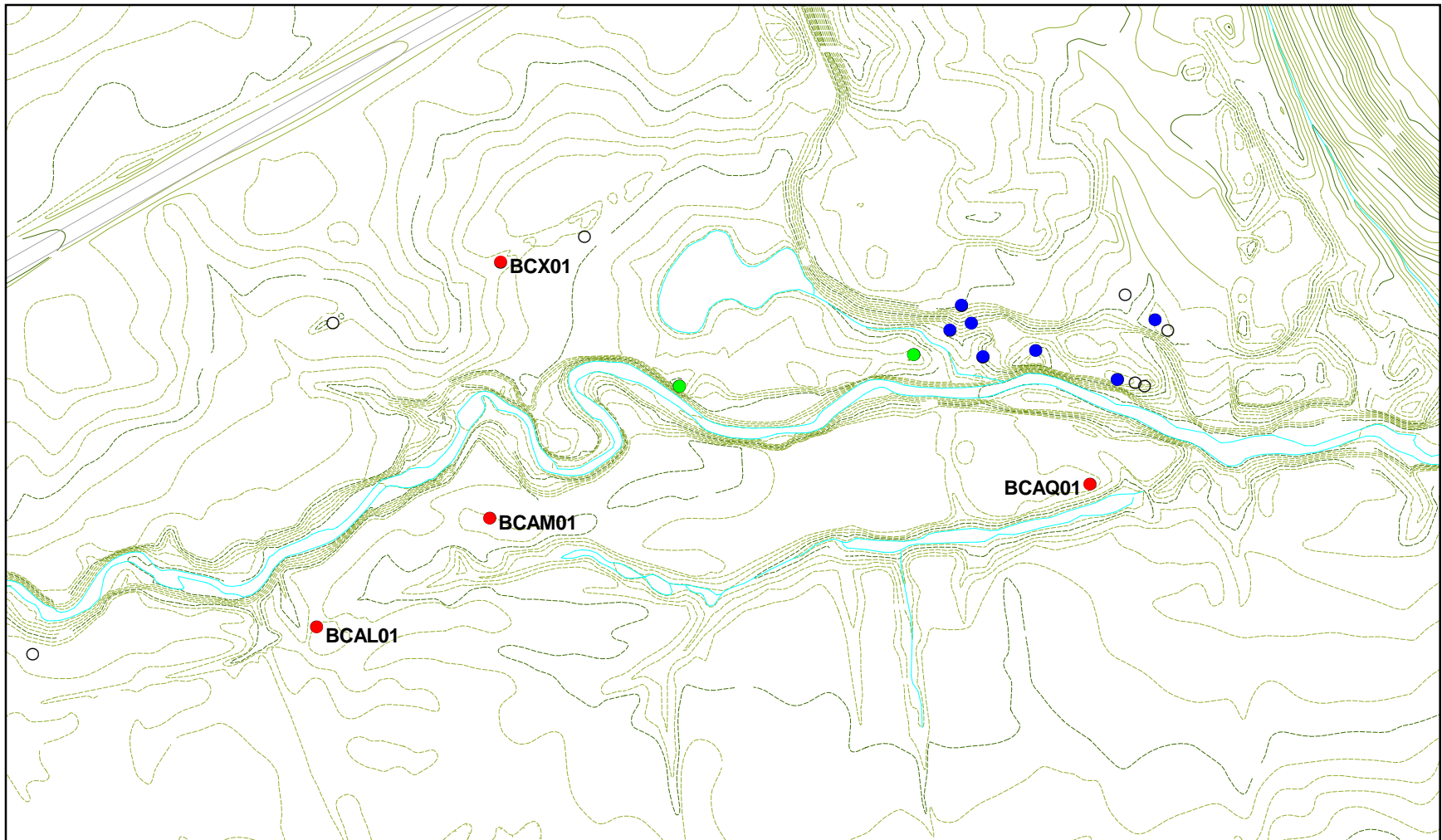
Figure B-27. (Continued) B-54
