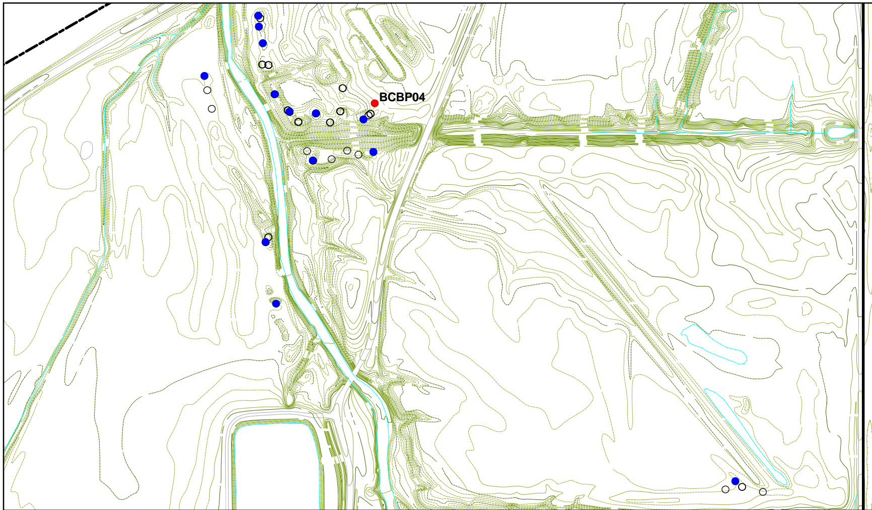
Figure B.18. (Continued) B-41
