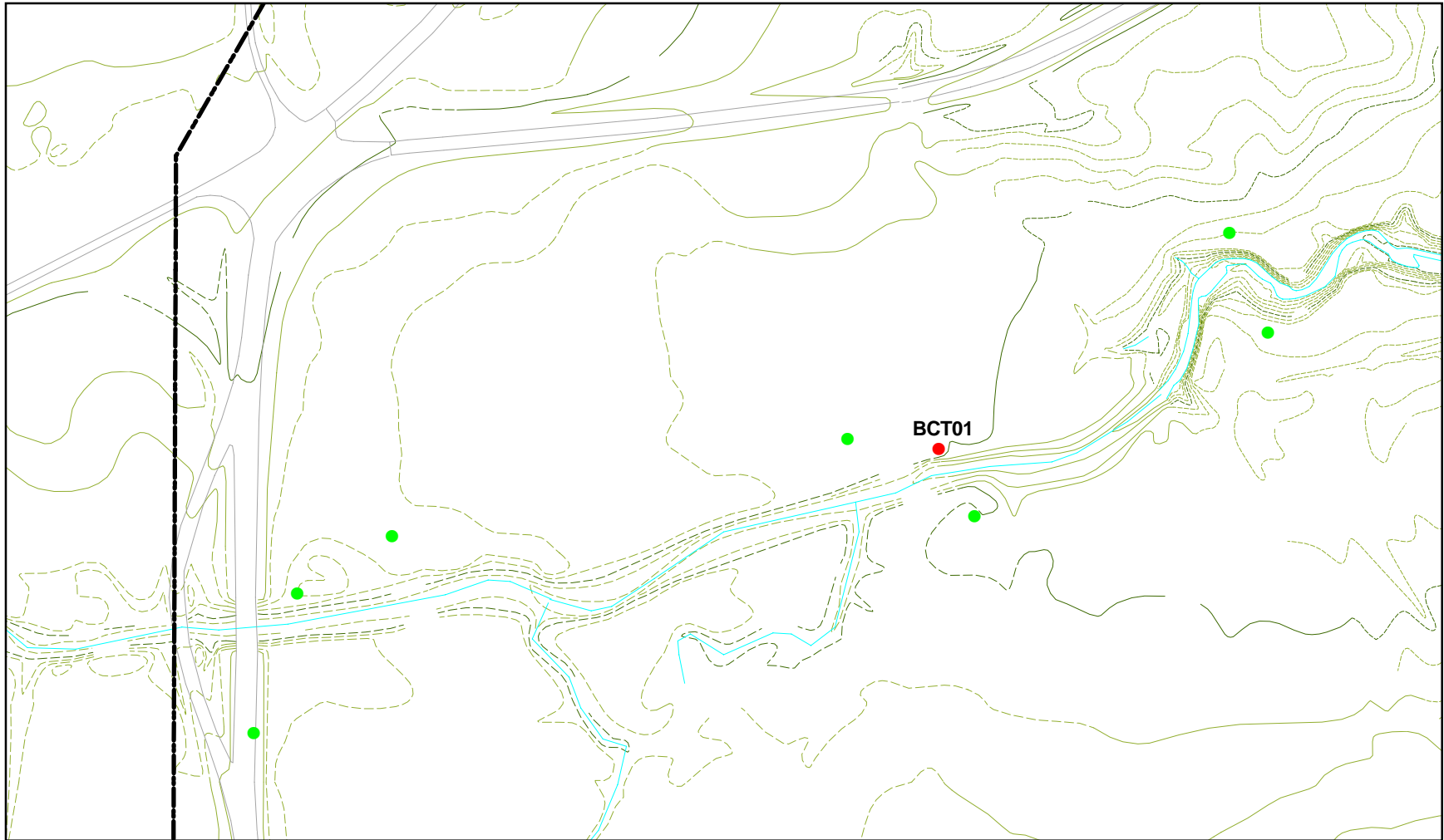
Figure B-29. (Continued) B-60
