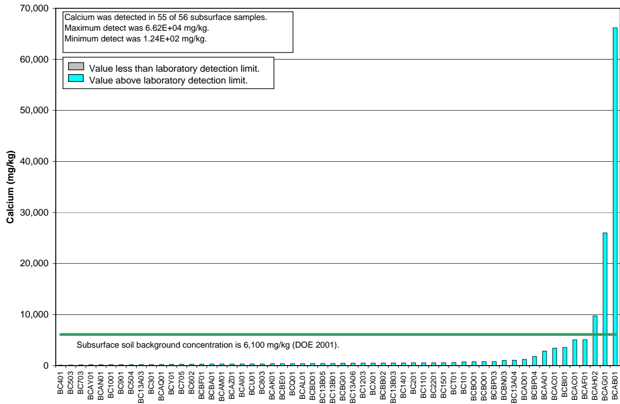
Figure B.11. Comparison between Calcium Concentrations in Samples from Soil Piles Addendum 2 and Subsurface Soil Background Concentrations
