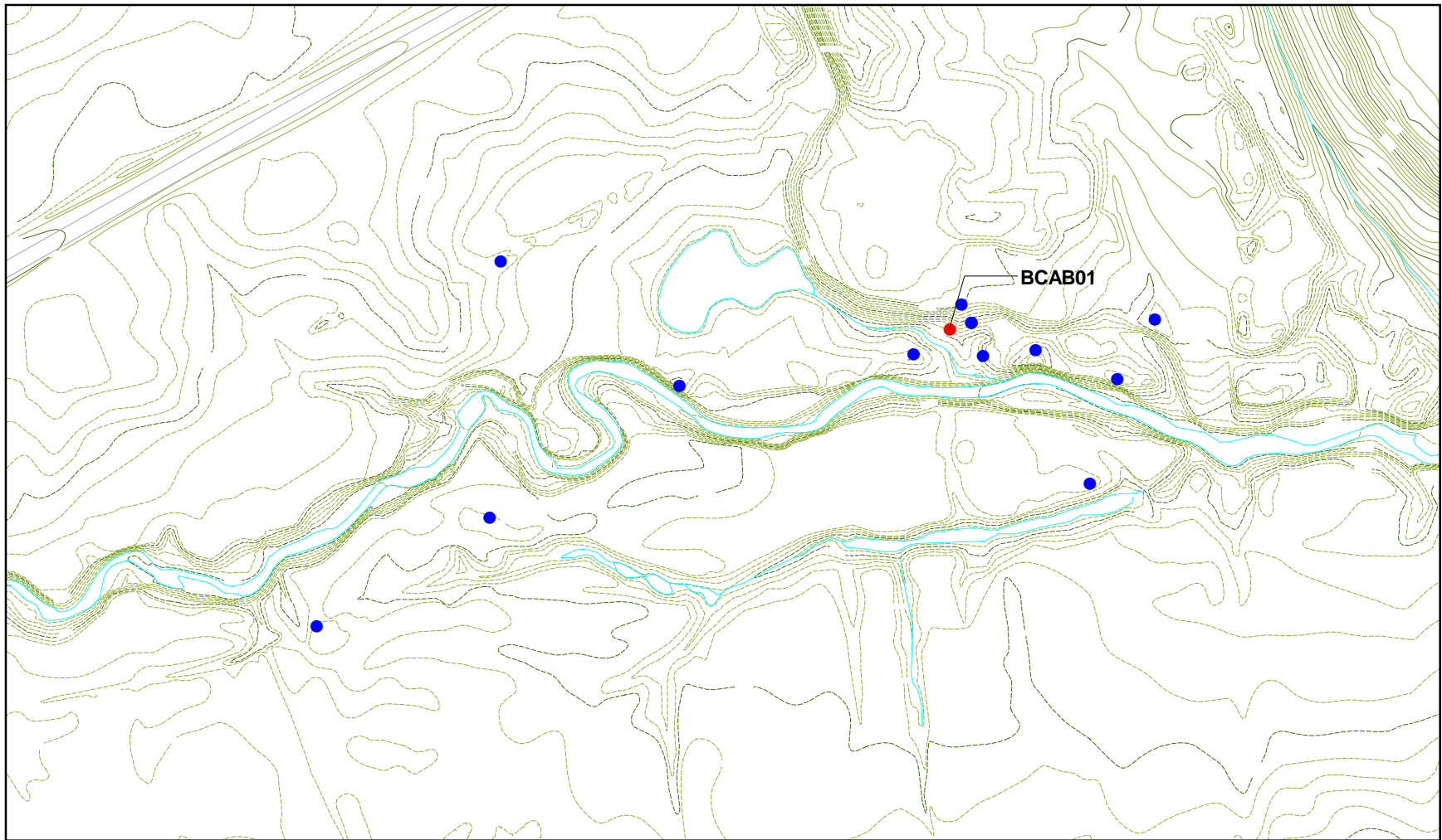
Figure B.4. (Continued) B-10
