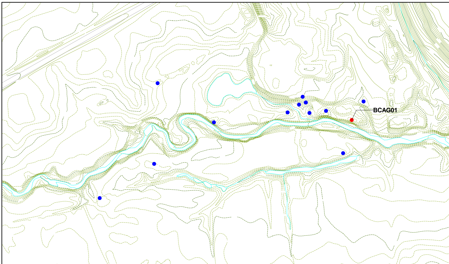
Figure B.2. (Continued) B-6
