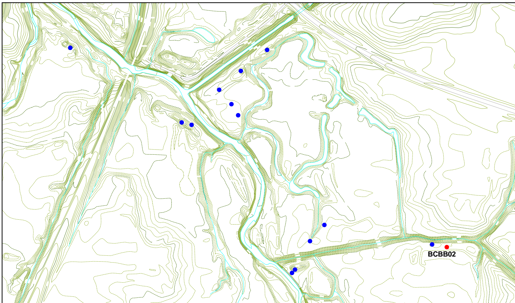
Figure B.2. (Continued) B-7
