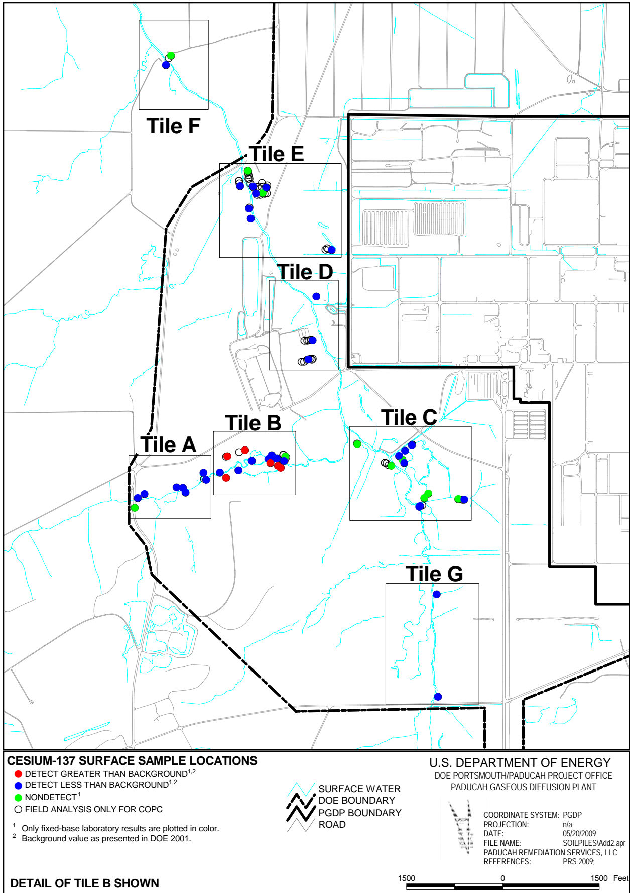
Figure B.24. Location of Sample Stations in Addendum 2 Soil Pile Sampling for Cesium-137 in the Surface B-49
