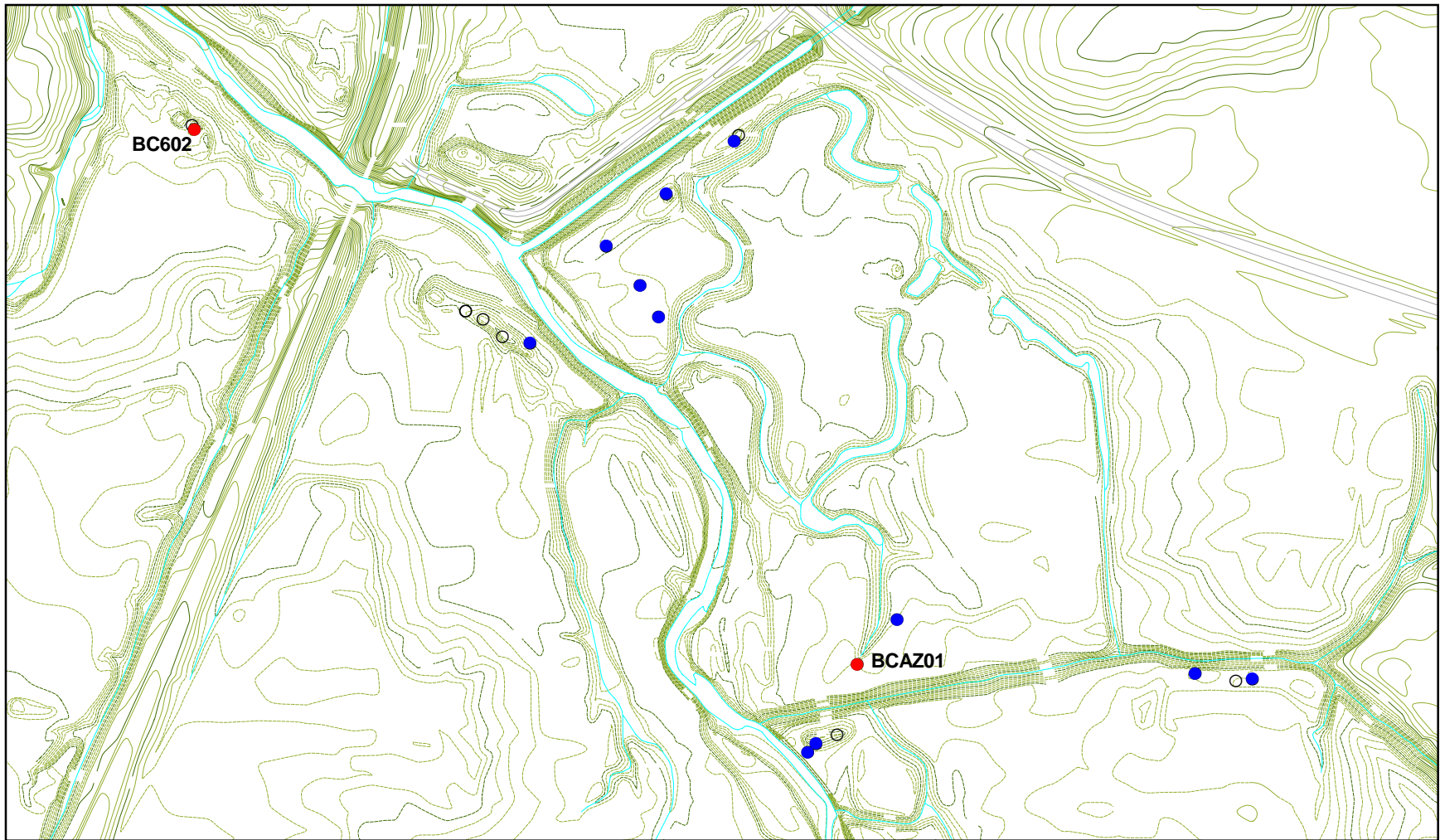
Figure B.14. (Continued) B-33
