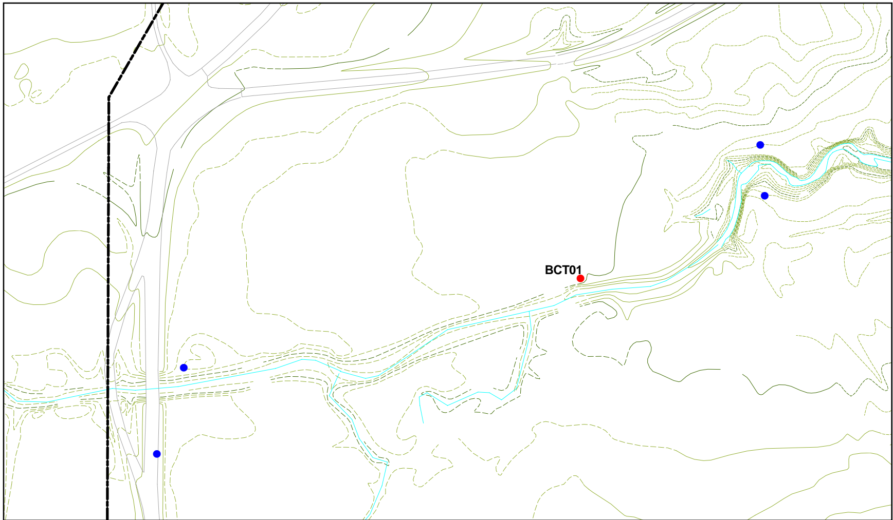
Figure B-22. (Continued) B-47
