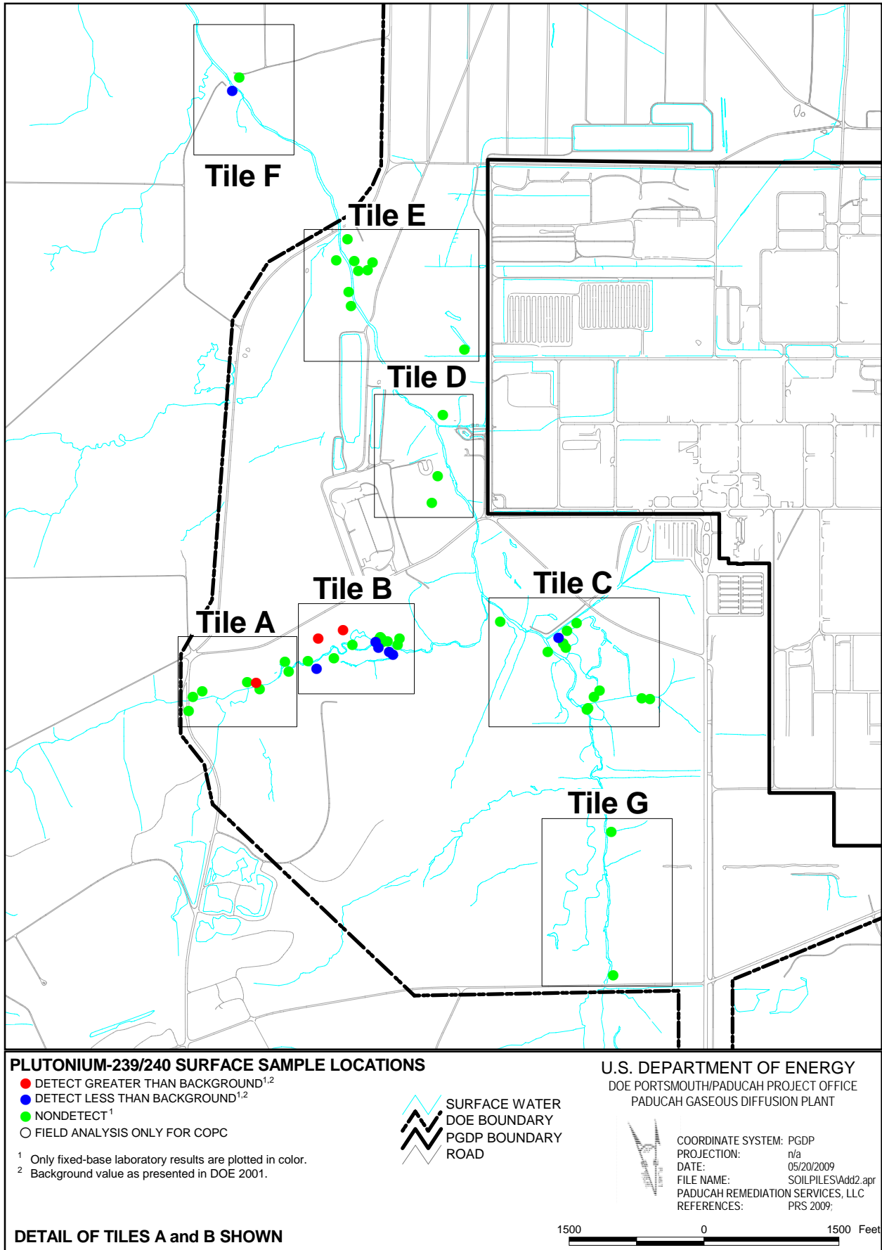
Figure B.29. Location of Sample Stations in Addendum 2 Soil Pile Sampling for Plutonium-239/240 on the Surface B-59
