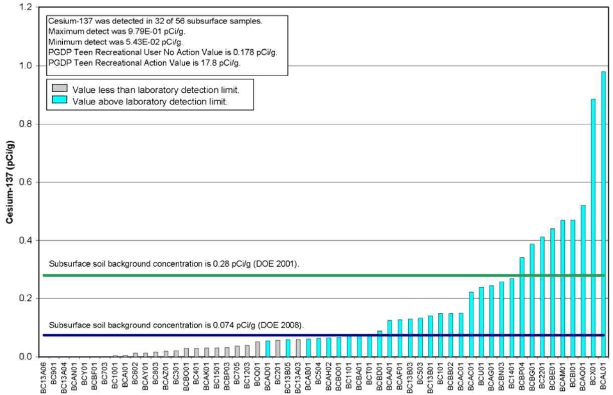
Figure B.26. Comparison between Cesium-137 Concentrations in Samples from Soil Piles Addendum 2 and Subsurface Soil Background Concentrations
