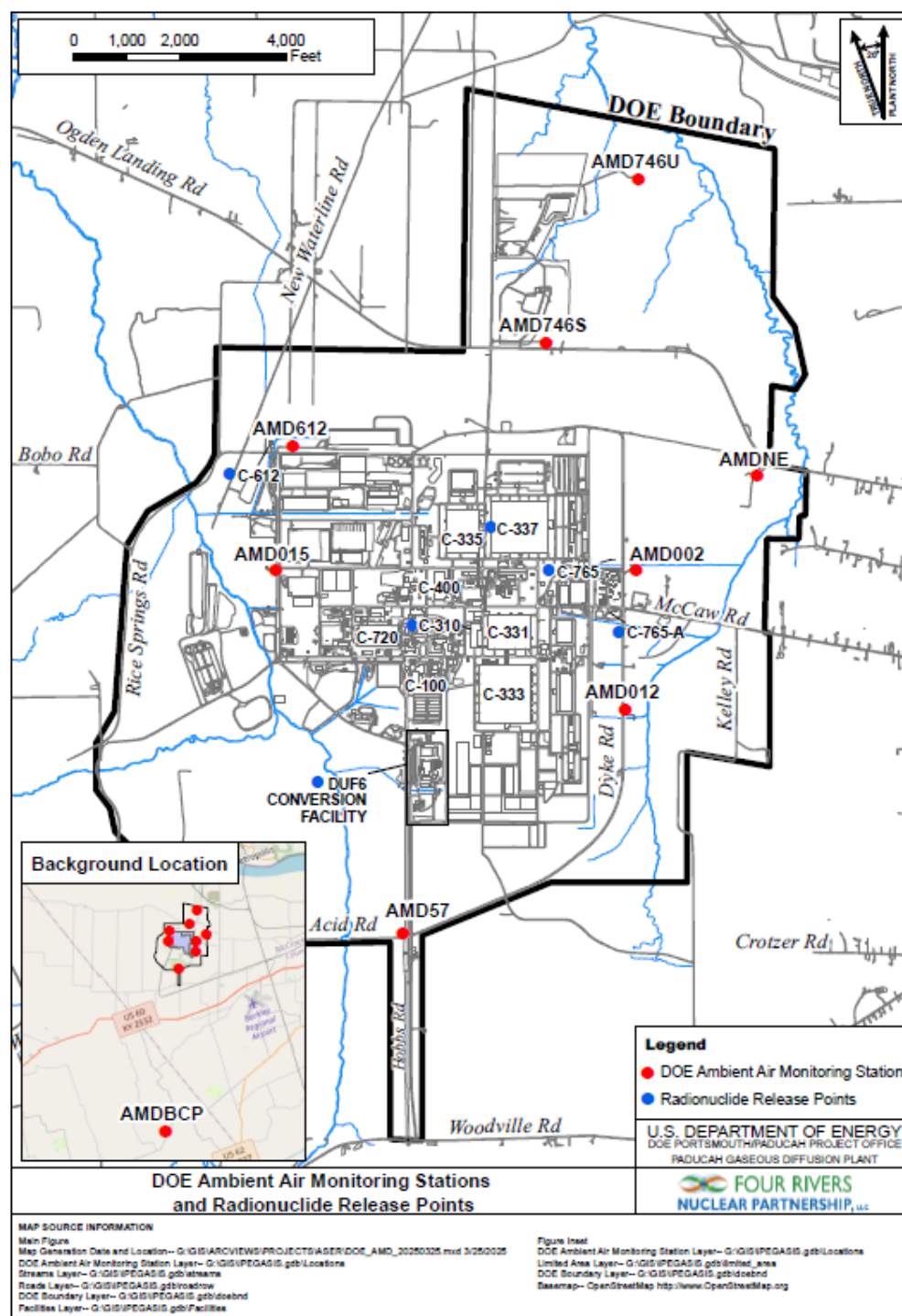
Figure 2. Locations of the DOE Ambient Air Monitoring Stations
