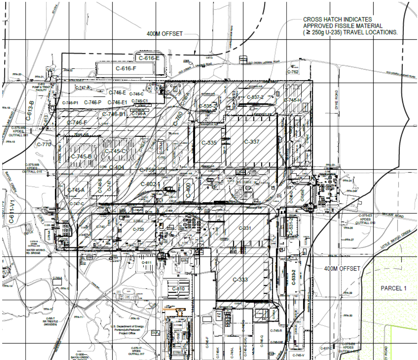
APPROVED FISSION MATERIAL ( \geq 250 g U-235) TRAVEL LOCATIONS – SITE PLAN
