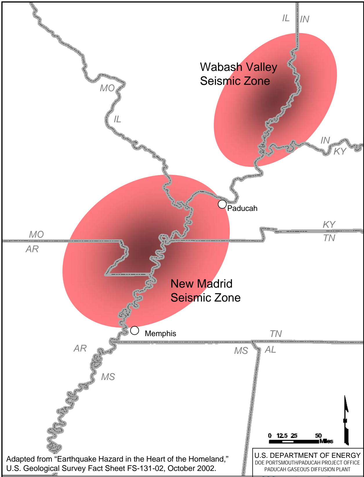
Figure 4.4. Regional Tectonic Map
