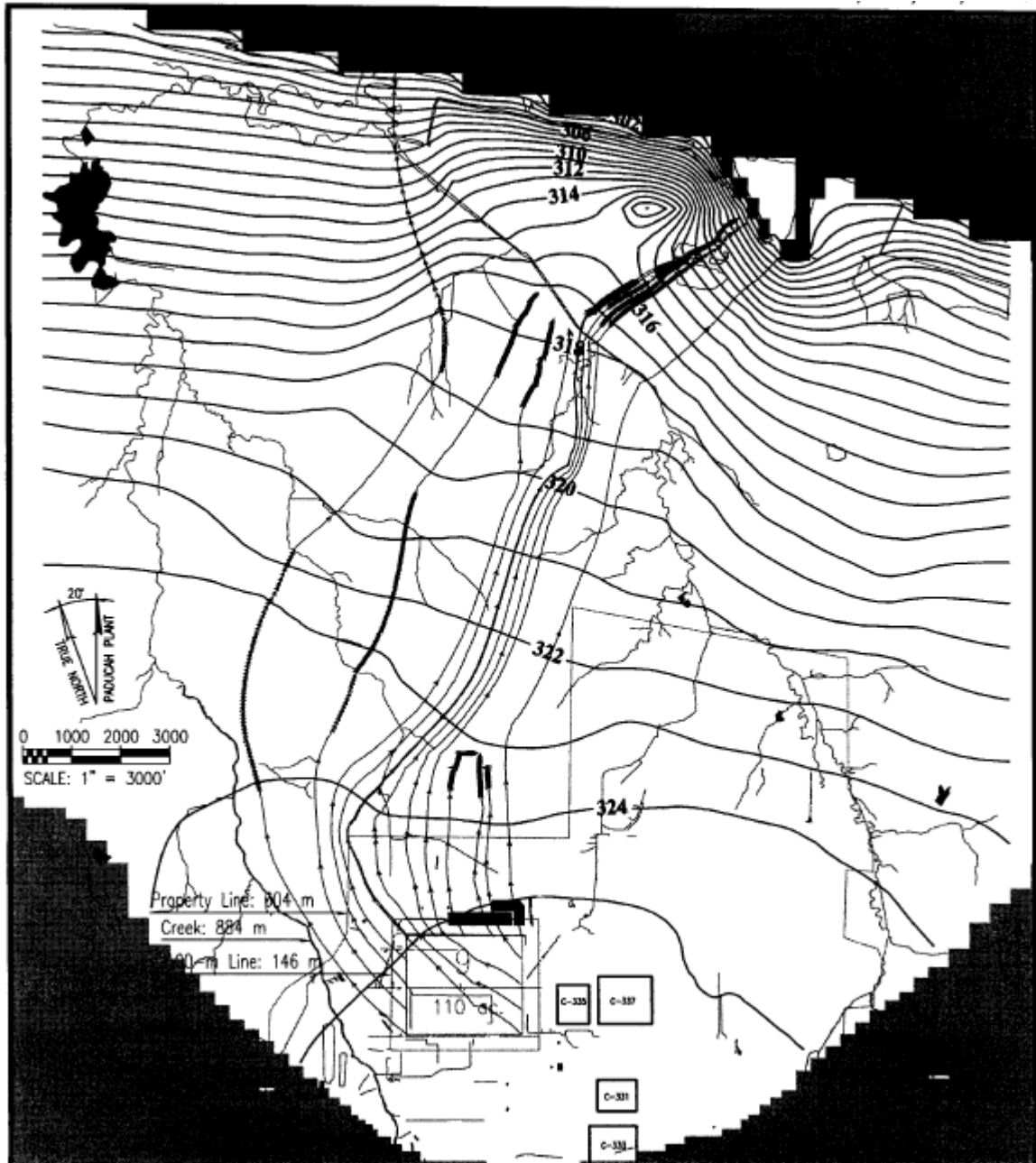
Figure C.2. Example Flow Paths from the Sitewide Groundwater Model
