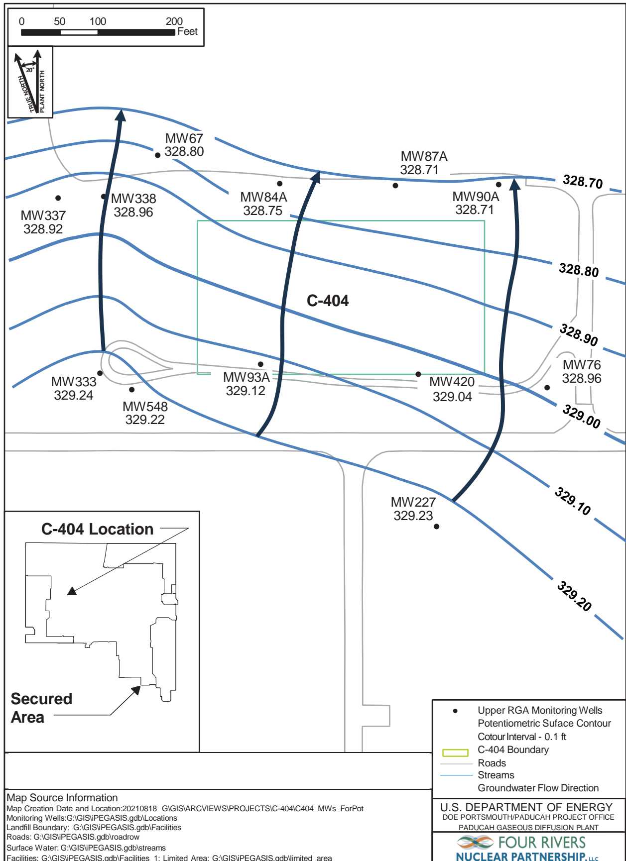
Figure C.2. Potentiometric Surface of the Upper Regional Gravel Aquifer at the C-404 Landfill July 22–23, 2025
