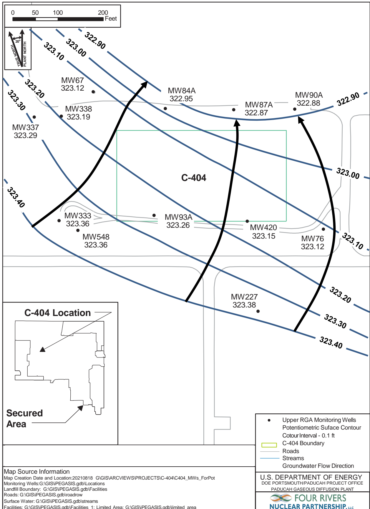
Figure C.1. Potentiometric Surface of the Upper Regional Gravel Aquifer at the C-404 Landfill January 21–22, 2025
