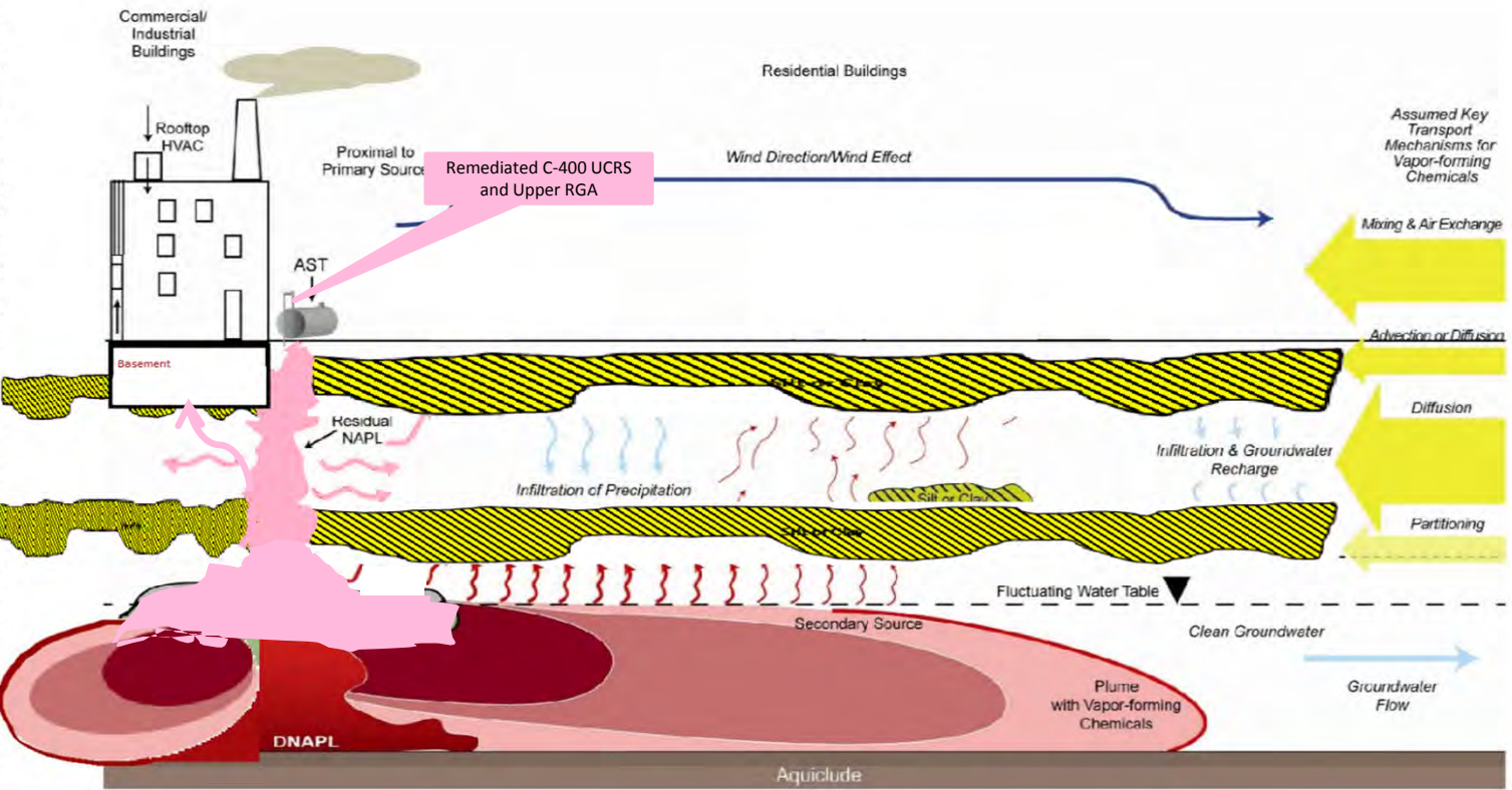
Figure 2-1 Illustration of Key Elements of the Conceptual Model of Soil Vapor Intrusion Note: Q_{soil} represents soil gas entry; Q_{air} represents air exchange.
