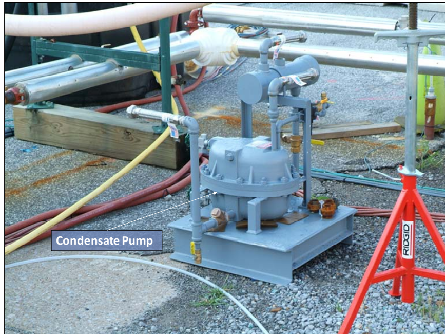
Figure 29. Condensate Pump
