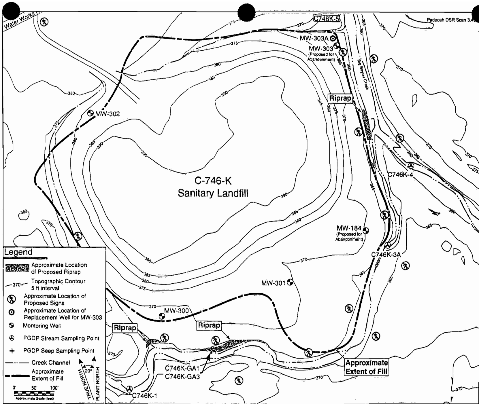
Fig. 3.43. Location of ROD remedial actions at the C-746-K Landfill (SWMU 8)
