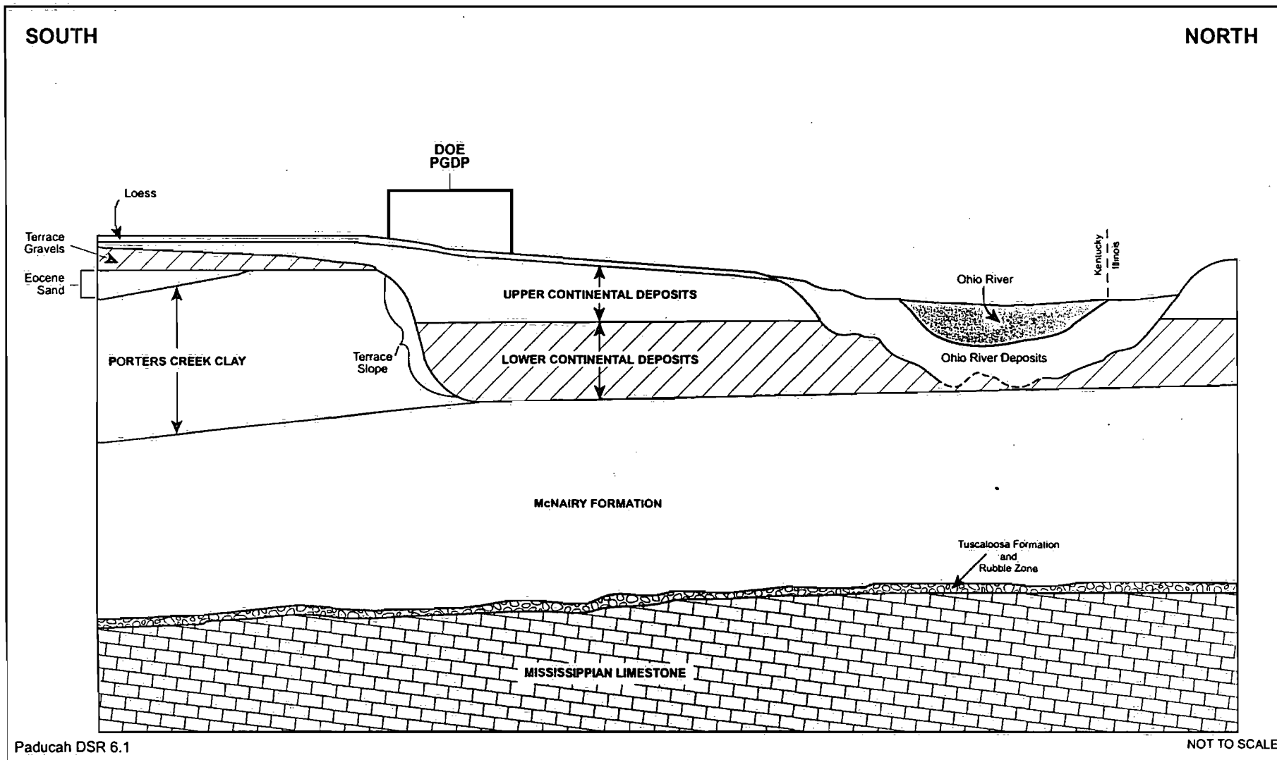
Fig. 6.2. Schematic of stratigraphic and structural relationships near the P GDP.
