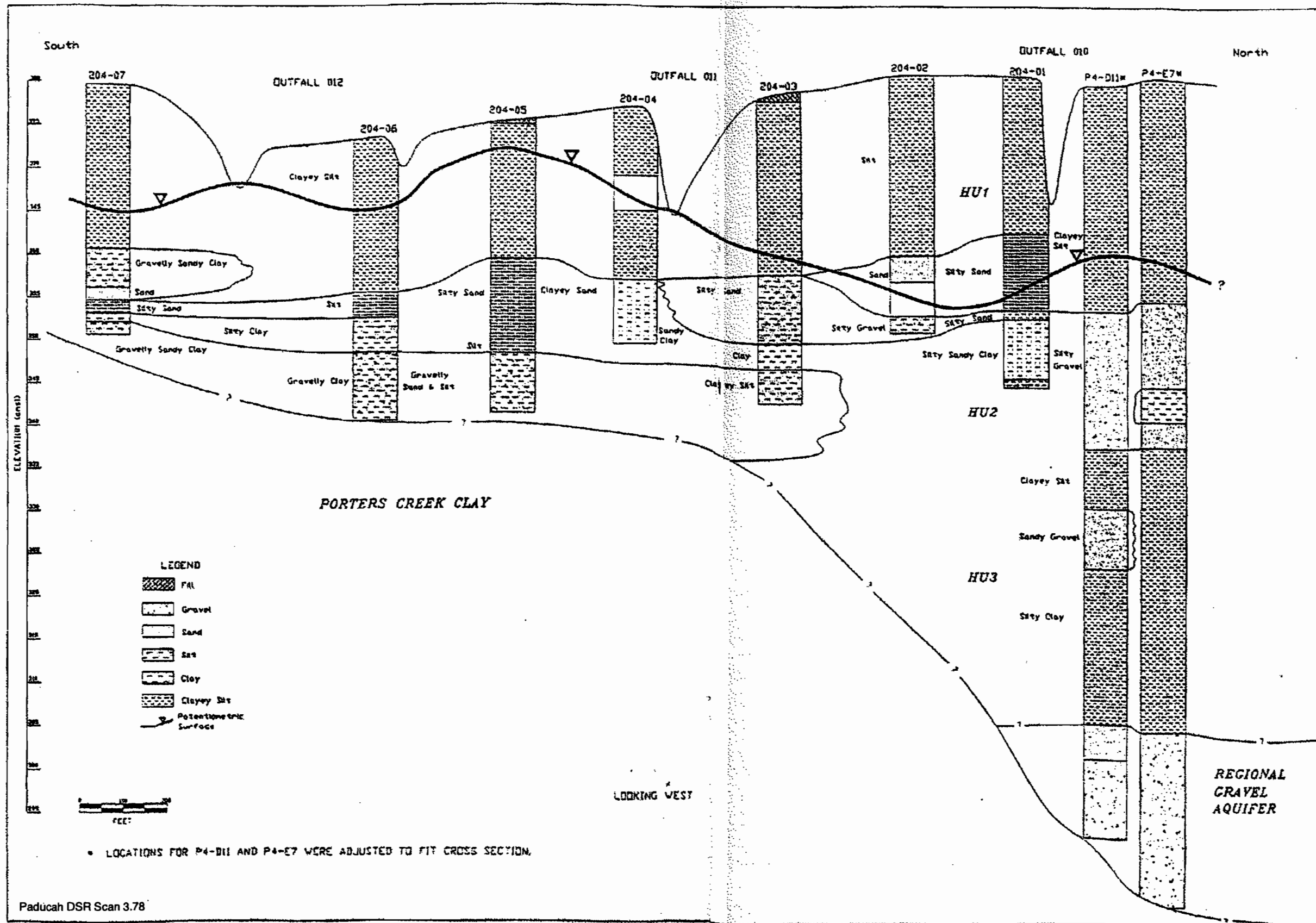
Fig. 3.78. Generalized geology/hydrogeology for the Outfalls 010 through 012 area.
