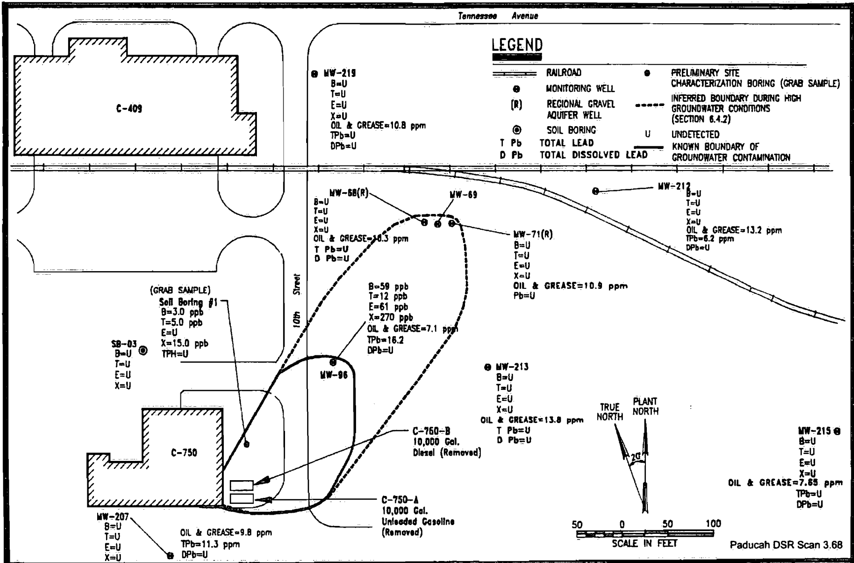
Fig. 3.68. Extent of BTEX contaminations in UCRS.
