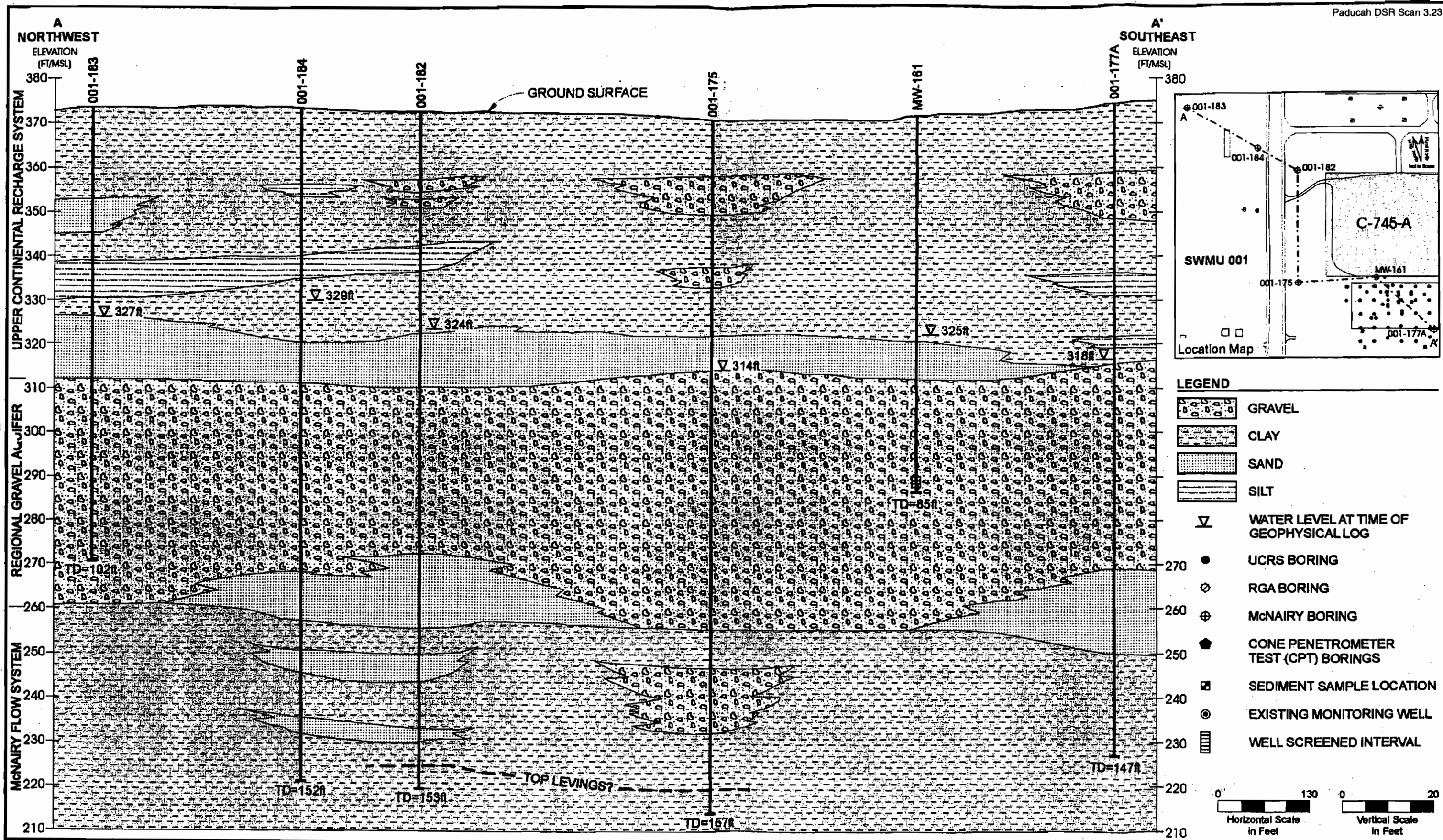
Fig. 3.23. Geologic cross section of SWMU 1.
