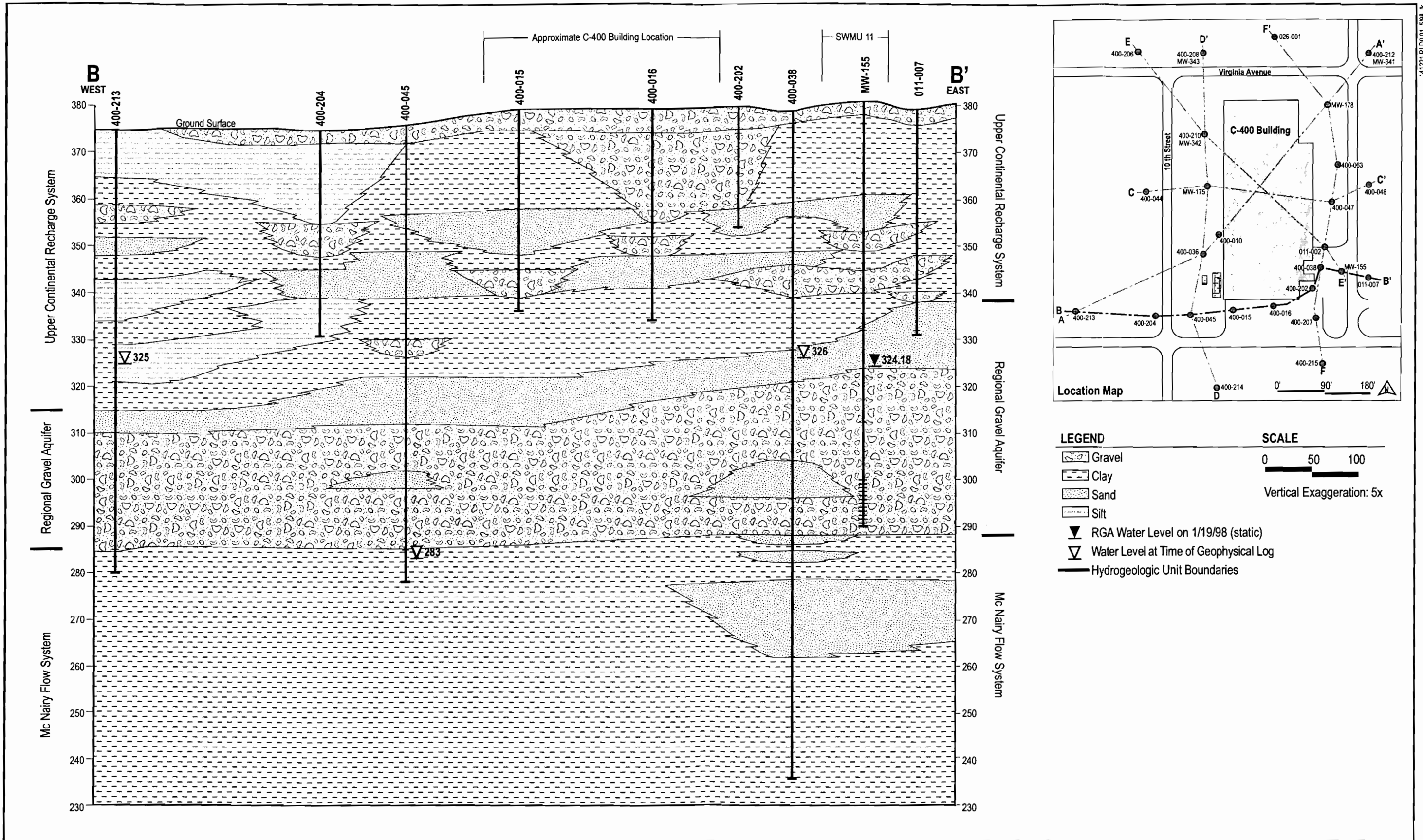
Fig. 3.9. East-west B-B' cross-section showing stratigraphy at WAG 6.
