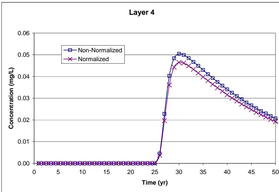
Figure E.3.8. Comparison of Predicted Groundwater Concentrations from a Layer 4 Source for TCE at SWMU 4 for the Normalized and Non-Normalized Area and Source Concentrations
