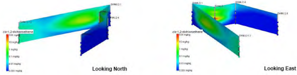
SWMU 2 cis -1,2-DCE: 0 – 20 ft bgs (Vertical Exaggeration = 2)
