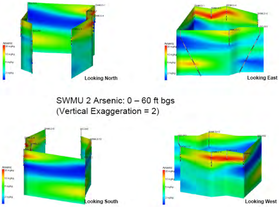
Figure E2.2. Arsenic Concentration Fence Diagrams for SWMU 2
