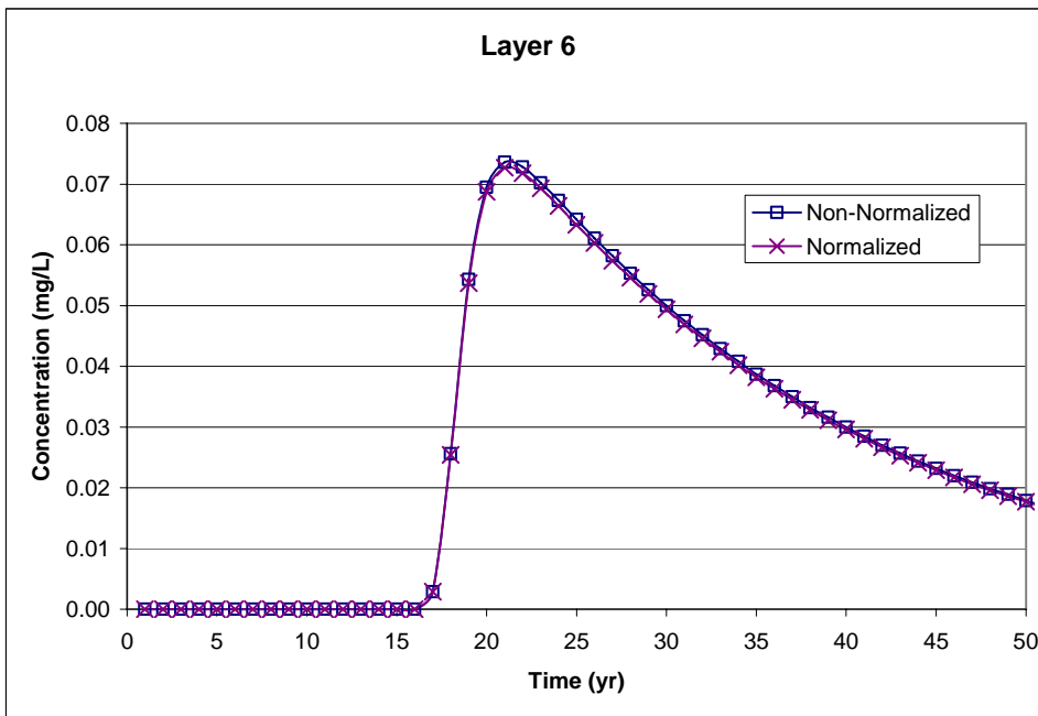
Figure E.3.10. Comparison of Predicted Groundwater Concentrations from a Layer 6 Source for TCE at SWMU 4 for the Normalized and Non-Normalized Area and Source Concentrations
