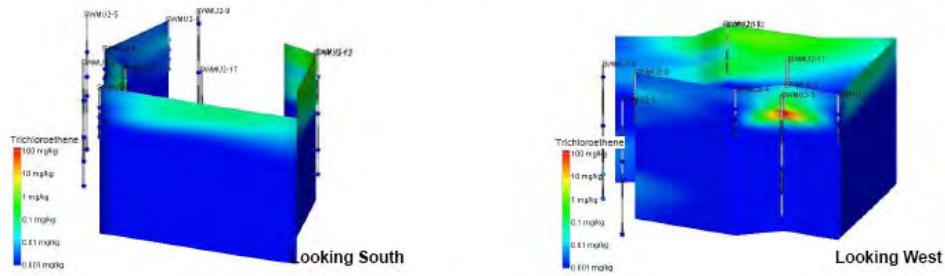
SWMU 2 TCE: 0 – 60 ft bgs (Vertical Exaggeration = 2)
