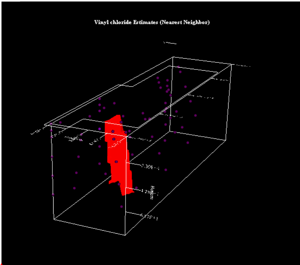
Figure E2.15. SWMU 7 Vinyl Chloride SADA Nearest Neighbor Interpolation Map (3-D)
