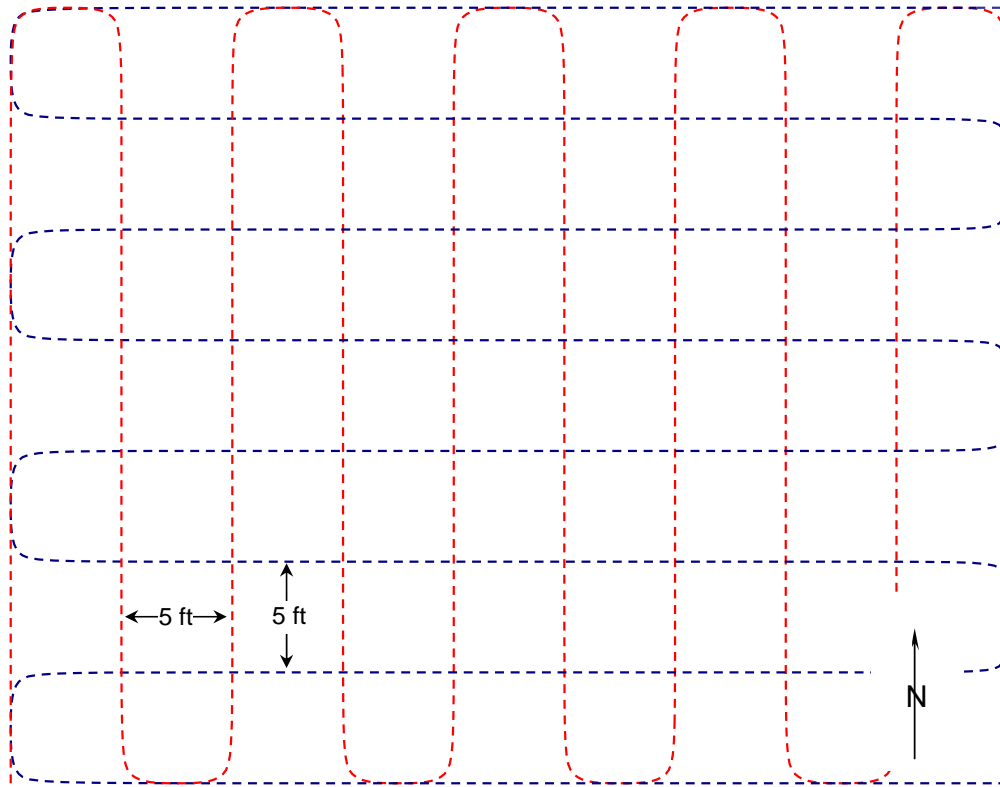
Figure A.1. Example EM-61 Survey Grid for BGOU RI
