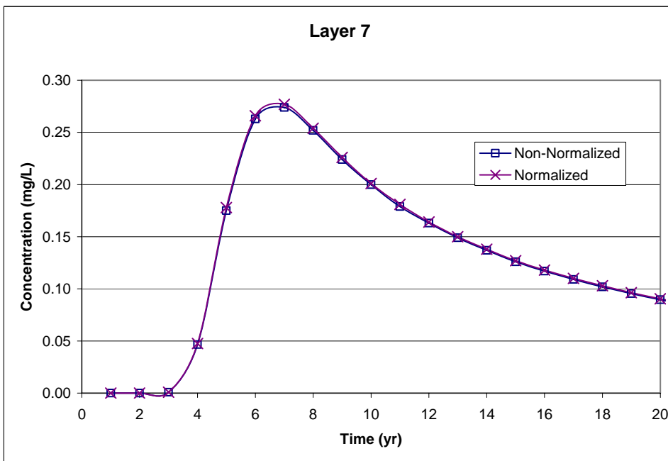
Figure E.3.11. Comparison of Predicted Groundwater Concentrations from a Layer 7 Source for TCE at SWMU 4 for the Normalized and Non-Normalized Area and Source Concentrations
