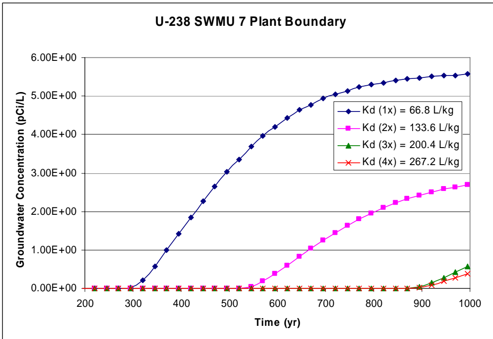
Figure E.3.14. SWMU 7 Groundwater Concentrations for ^{238}\text{U} at the Plant Boundary for Varying UCRS K_d Values
