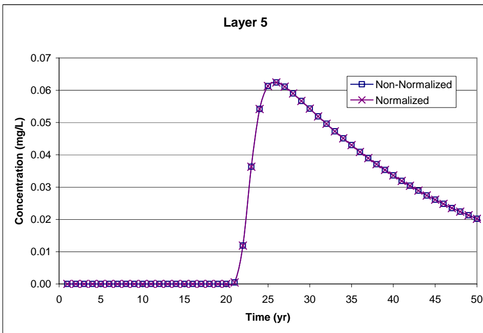
Figure E.3.9. Comparison of Predicted Groundwater Concentrations from a Layer 5 Source for TCE at SWMU 4 for the Normalized and Non-Normalized Area and Source Concentrations
