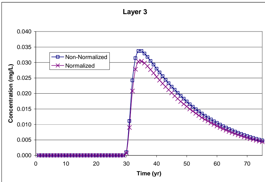
Figure E.3.7. Comparison of Predicted Groundwater Concentrations from a Layer 3 Source for TCE at SWMU 4 for the Normalized and Non-Normalized Area and Source Concentrations
