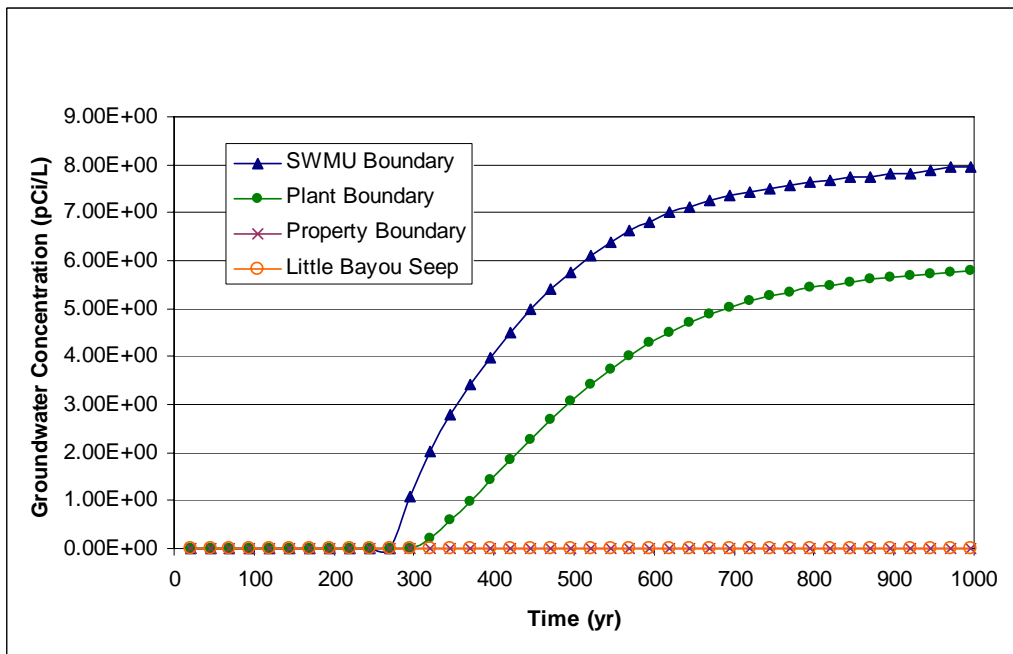
Figure 5.24. Predicted 234 U Activities in Groundwater at the POEs Based on Contaminant Leaching from SWMU 7
