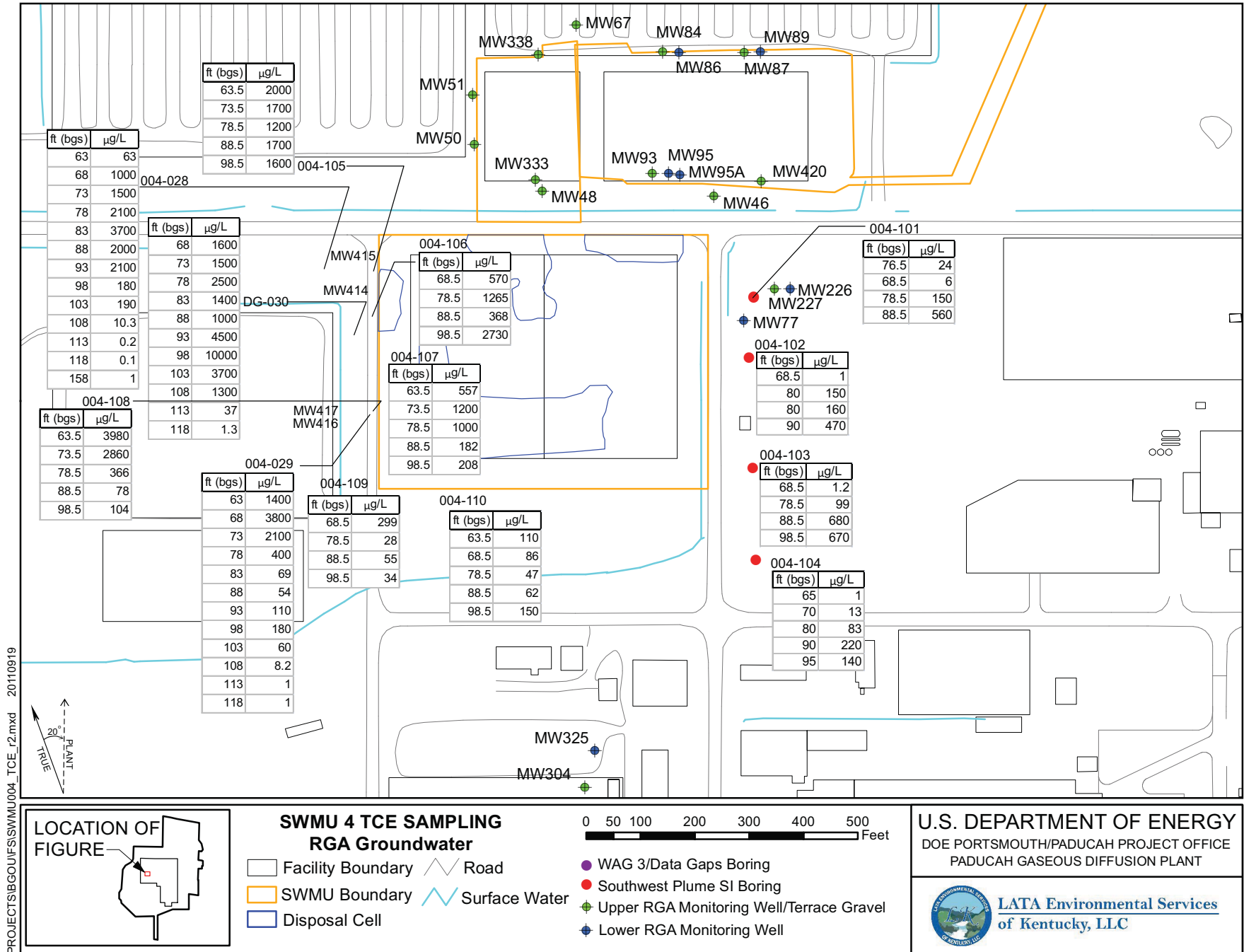
Figure 8. TCE Distribution in Temporary Borings in the Vicinity of SWMU 4
