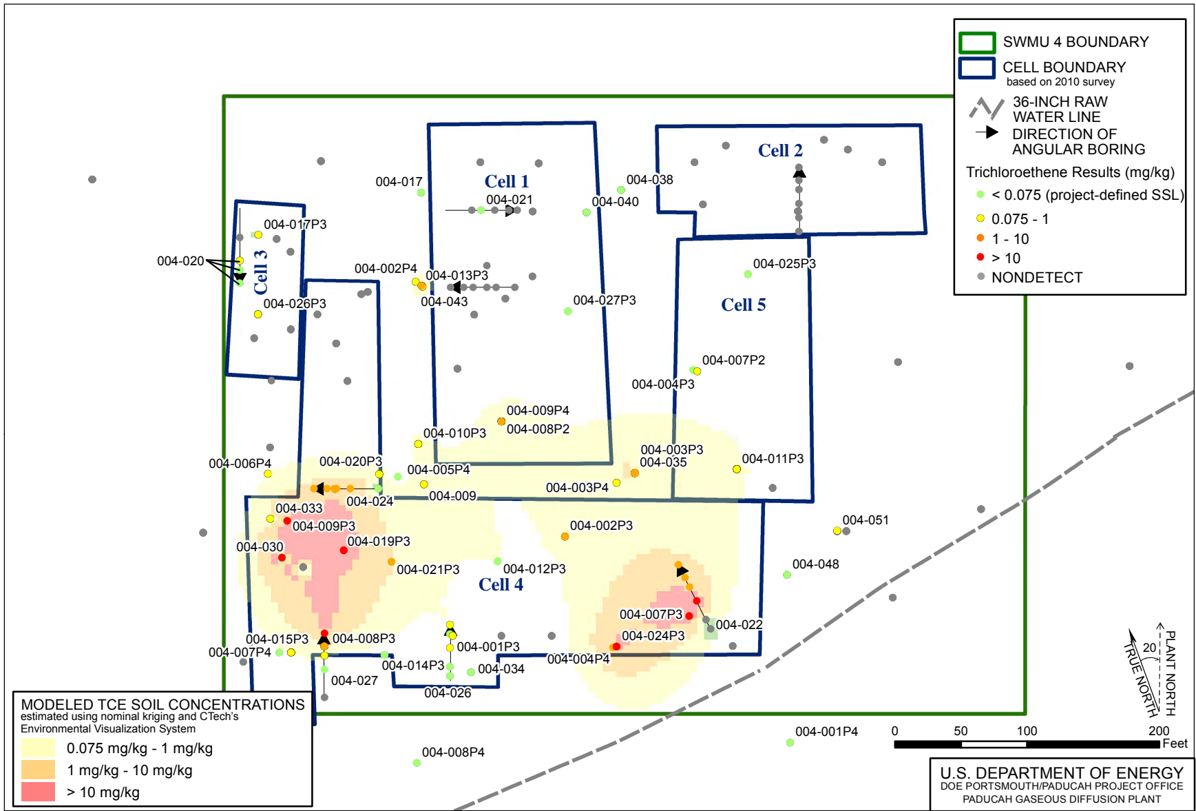
Figure 4.6. BGOU RI Addendum Subsurface Soil Trichloroethene Results
