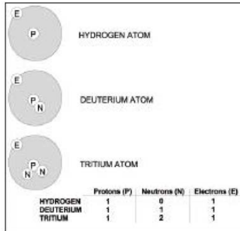
Figure A.1. Isotopes of the Element Hydrogen
