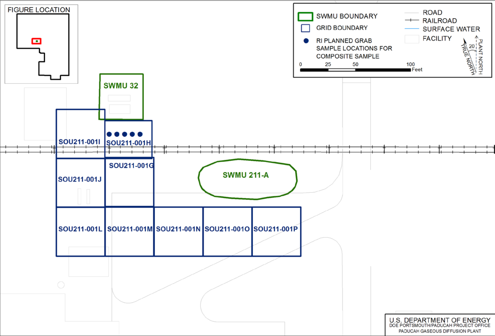
Figure 9. SWMU 211-A Soil Sampling Grids
