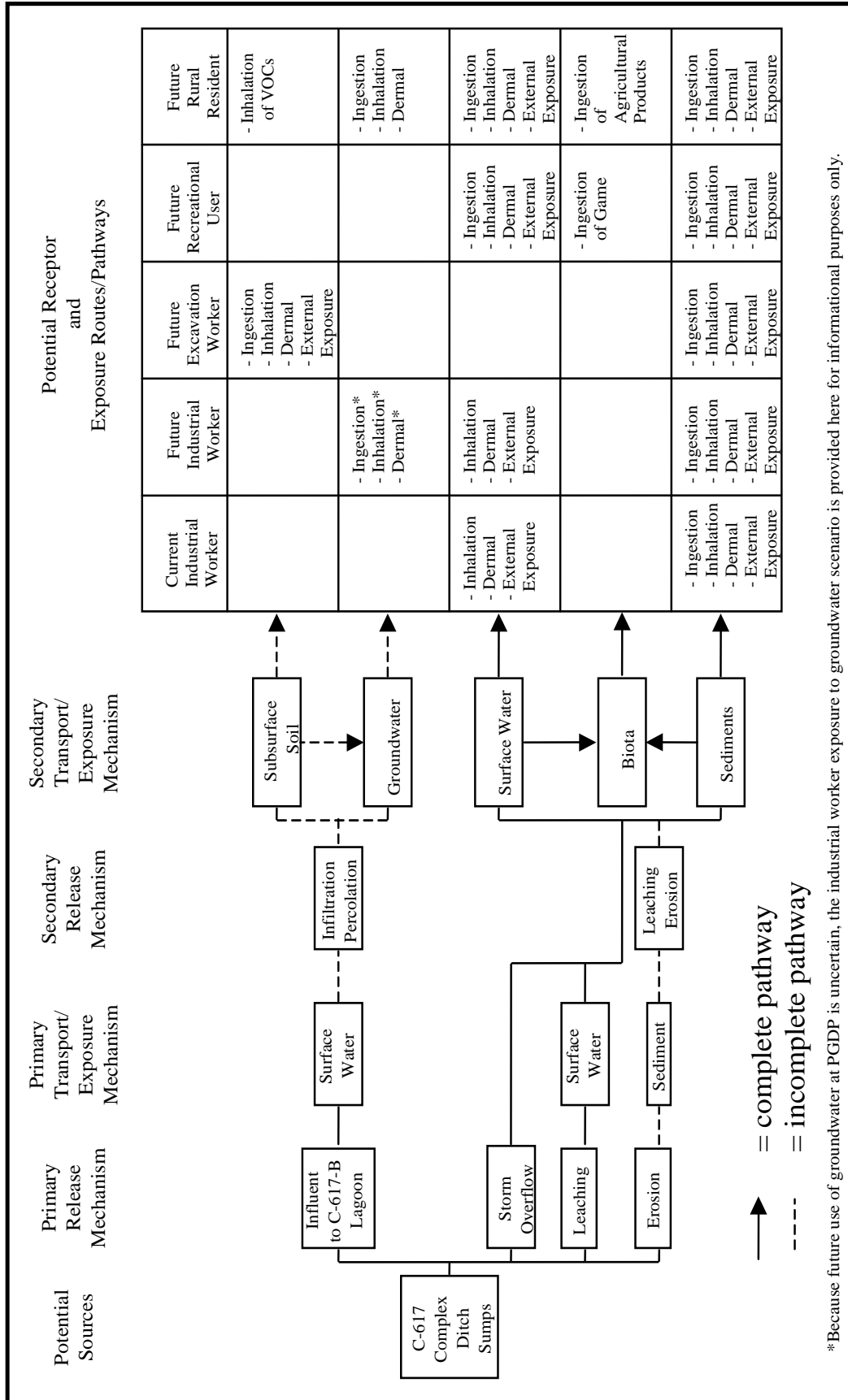
Figure 3.1. Example Risk-Based Conceptual Site Model
