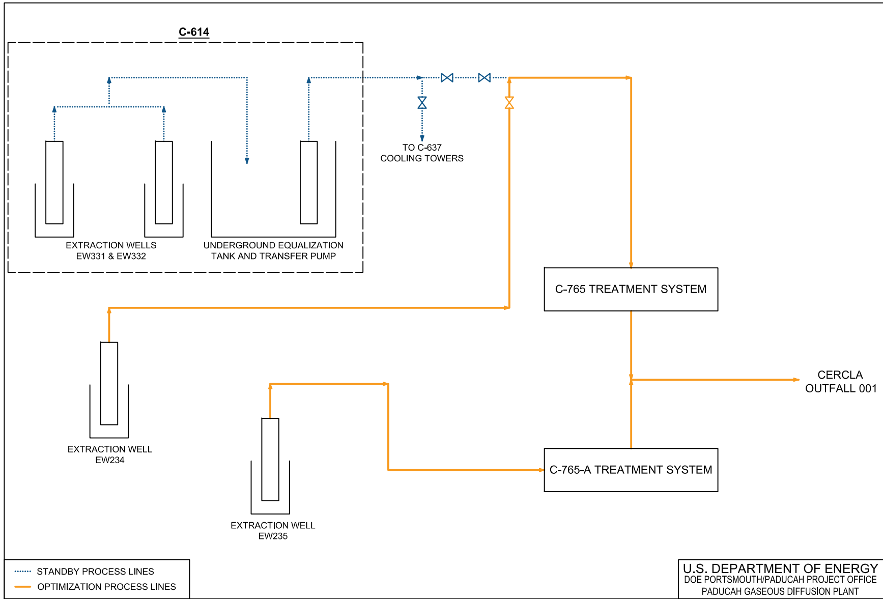
Figure 4. System Process Flow Diagram for NEPCS
