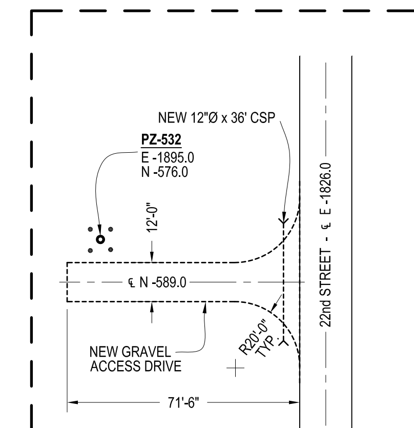
PZ532 ACCESS ROAD DETAIL
