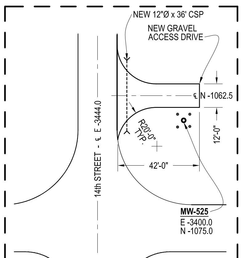
MW525 ACCESS ROAD DETAIL
