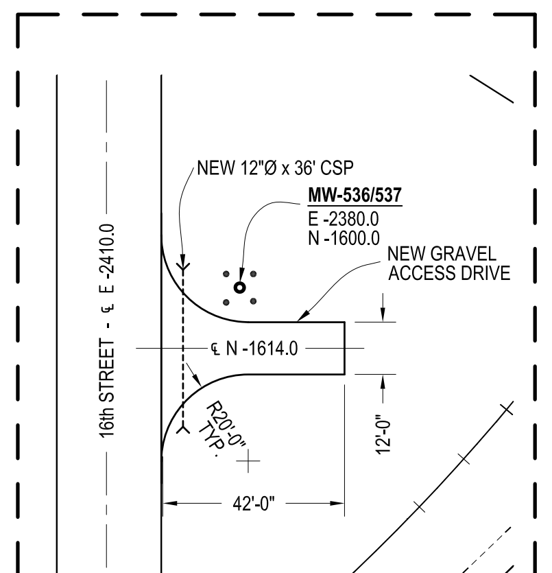
MW536/537 ACCESS ROAD DETAIL
