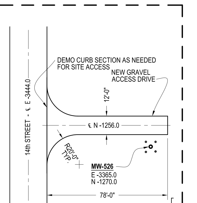
MW526 ACCESS ROAD DETAIL
