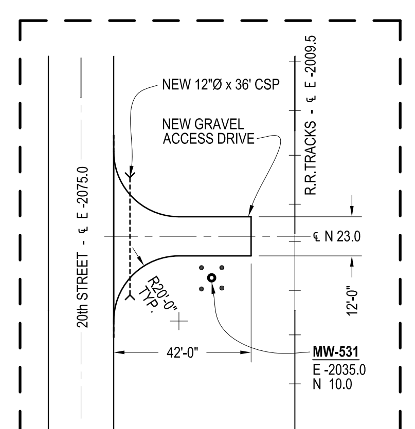
MW531 ACCESS ROAD DETAIL
