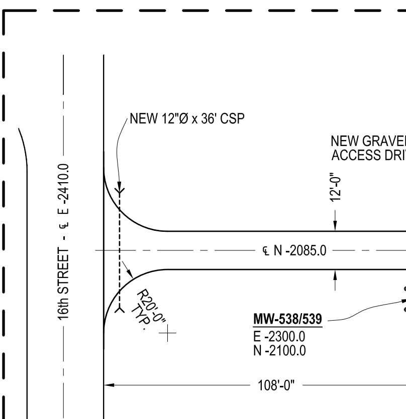
MW538/539 ACCESS ROAD DETAIL
