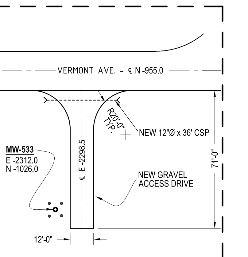
MW533 ACCESS ROAD DETAIL
