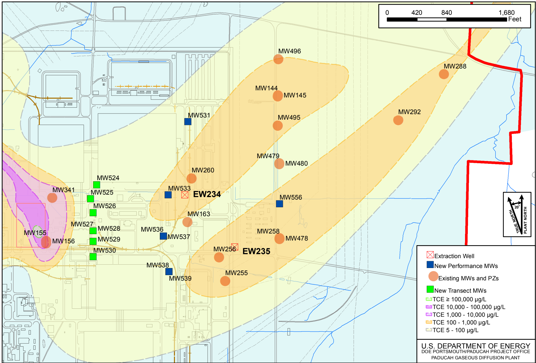
Figure 5. Northeast Plume Chemical Monitoring Network
