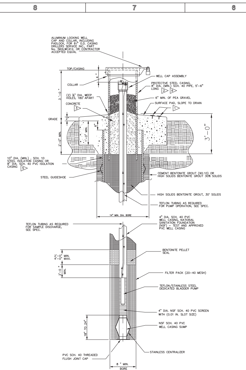
MONITORING WELL WITH ISOLATION CASING
