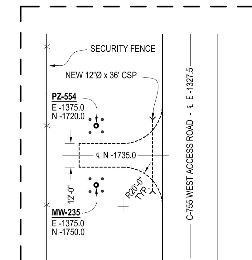
PZ554 & MW235 ACCESS ROAD DETAIL
