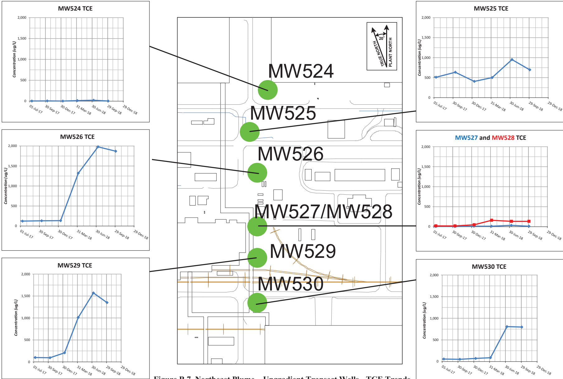
Figure B.7. Northeast Plume—Upgradient Transect Wells - TCE Trends
