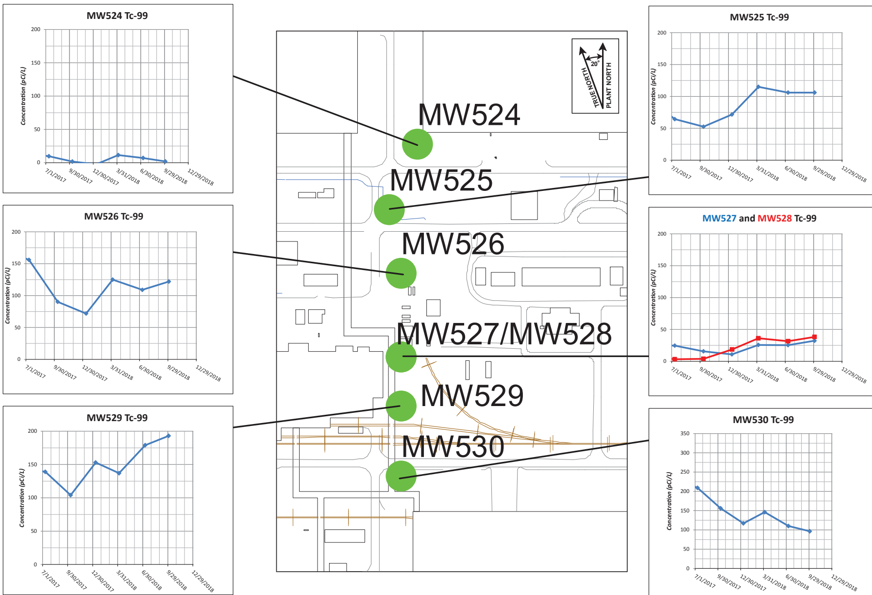
Figure B.8. Northeast Plume—Upgradient Transect Wells – Tc-99 Trends
