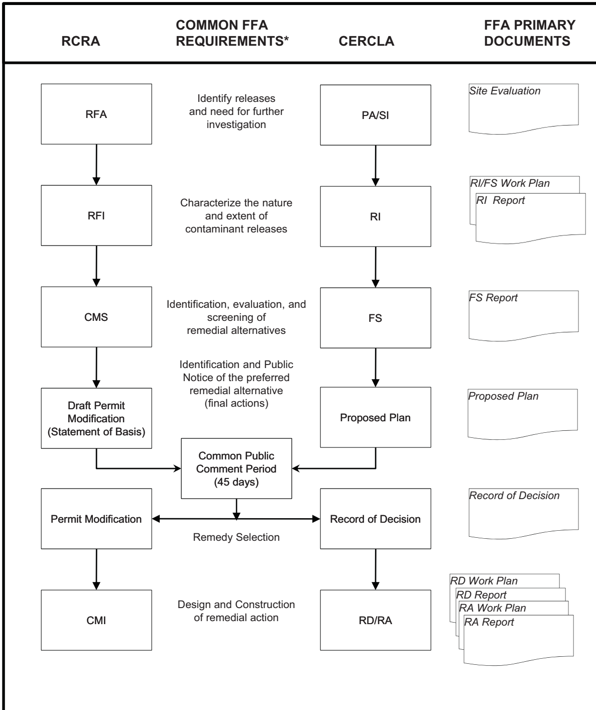
Figure 9. Diagram of Coordination of CERCLA and RCRA Process in Final Remedial Actions
